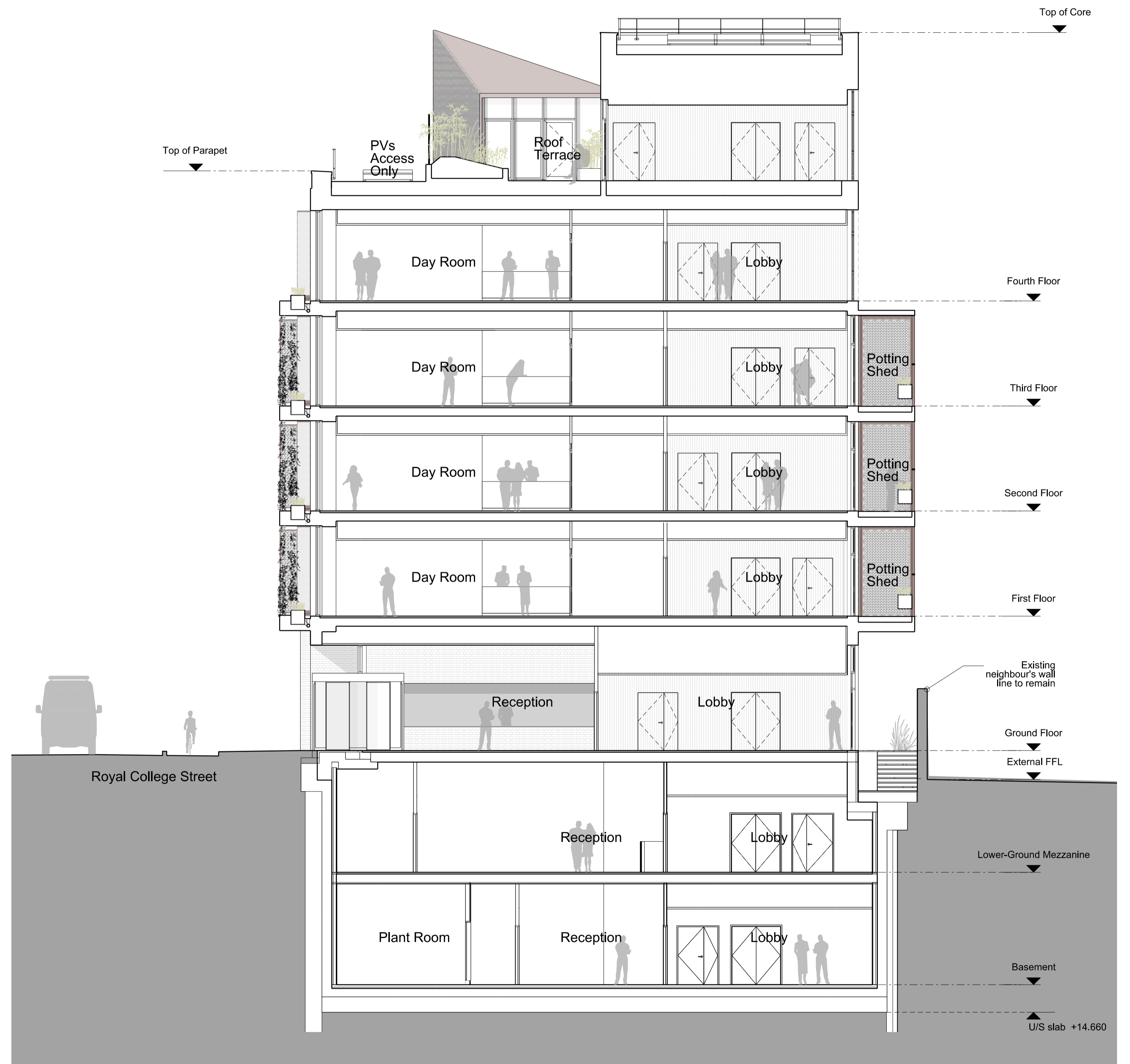
Section CC PROPOSED
