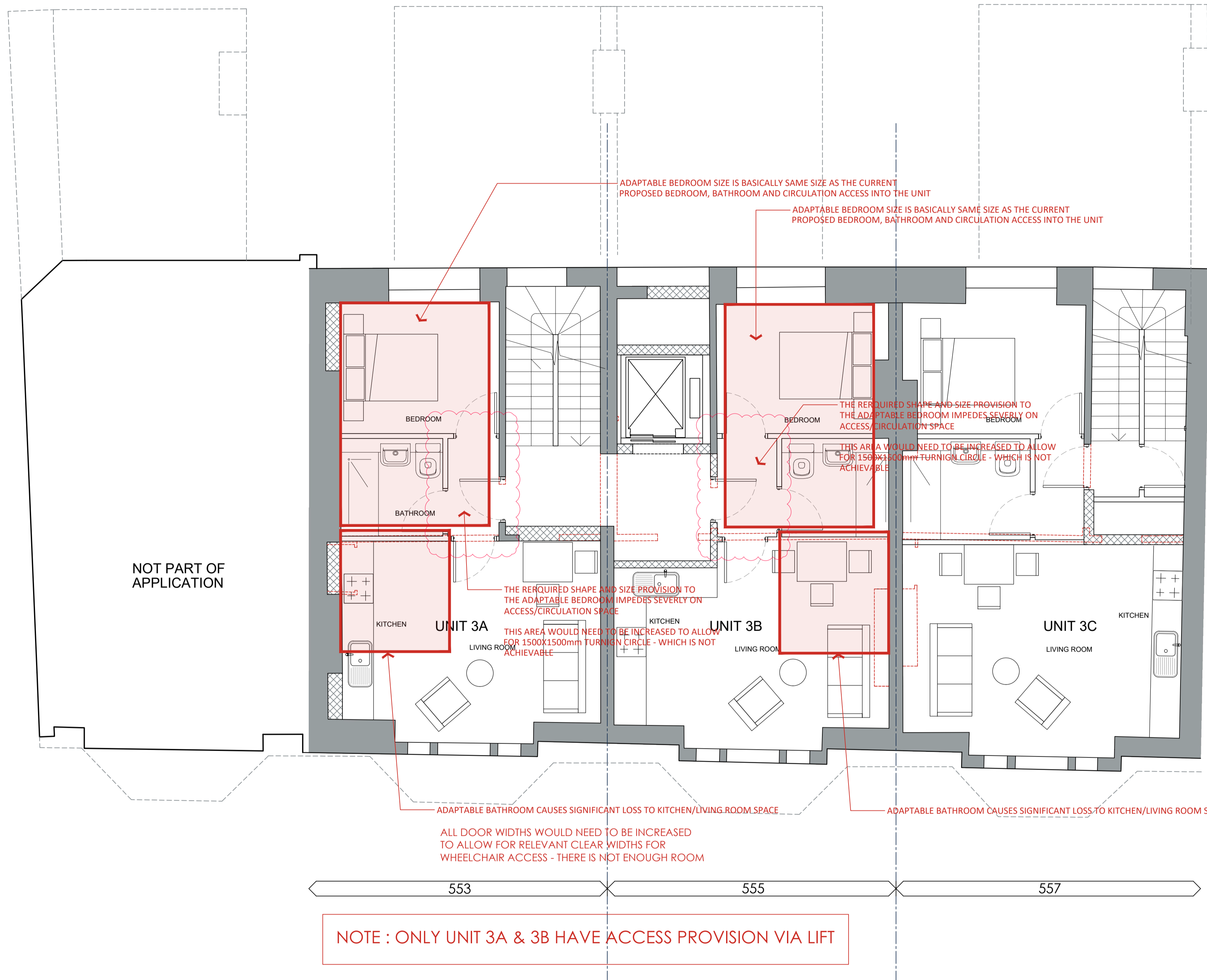
1 THIRD FLOOR - AS PROPOSED Scale: 1:50
