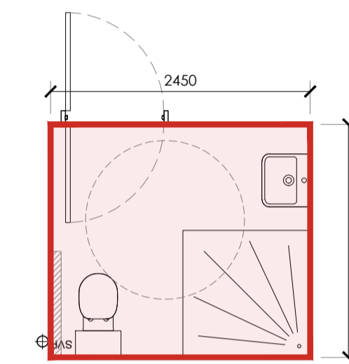
2 AD Part M4(3) Adaptable Bathroom Diagram 3.16C Scale: 1:50
