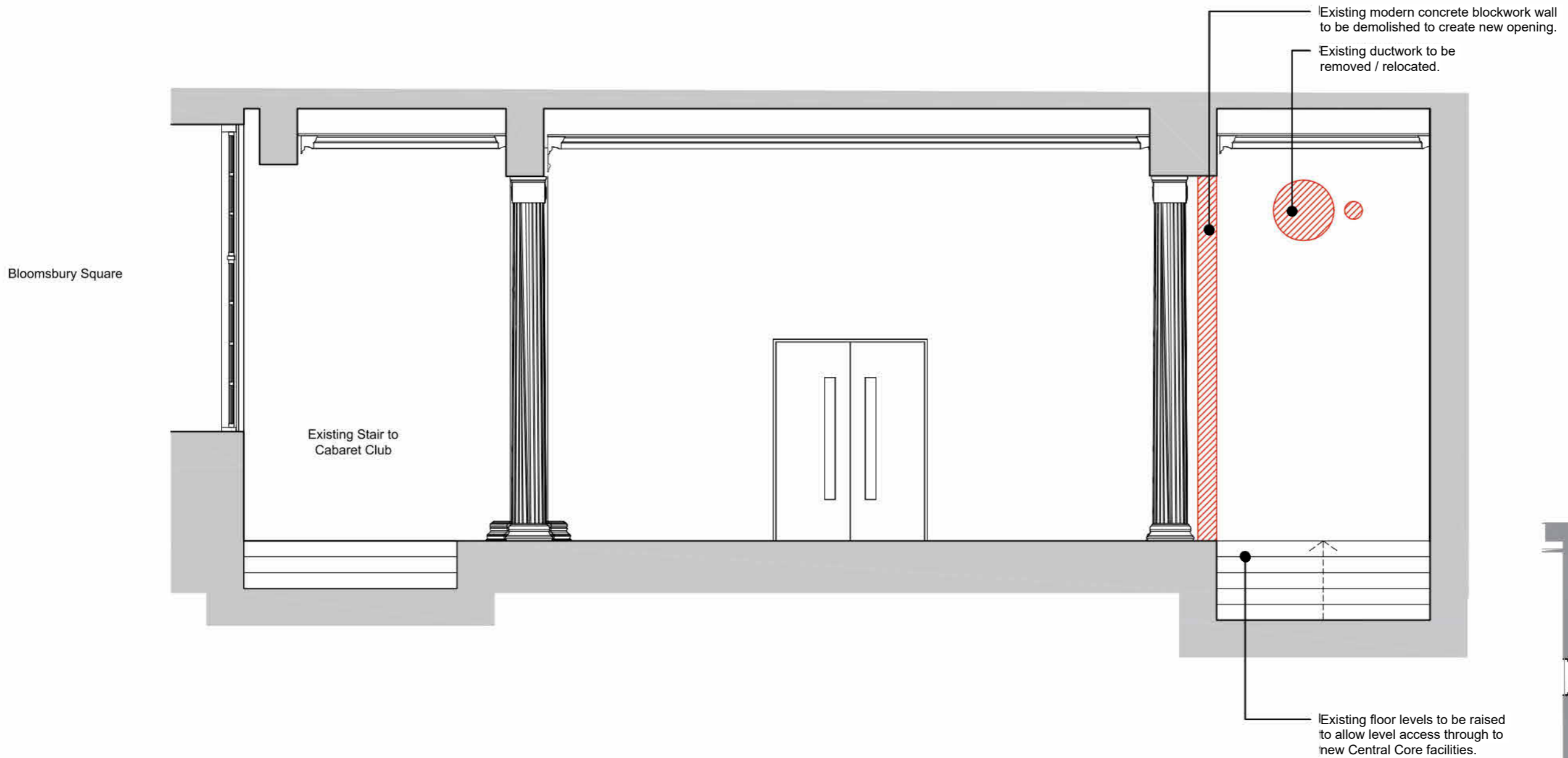
1 Historic Vestibule Basement Level B1 - North Elevation 1 : 10
