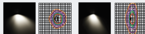
Flood Light Optic
