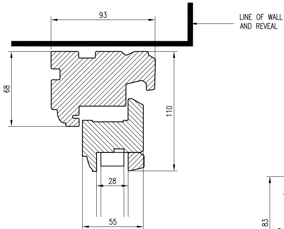
HEAD SECTION SCALE 1:2
