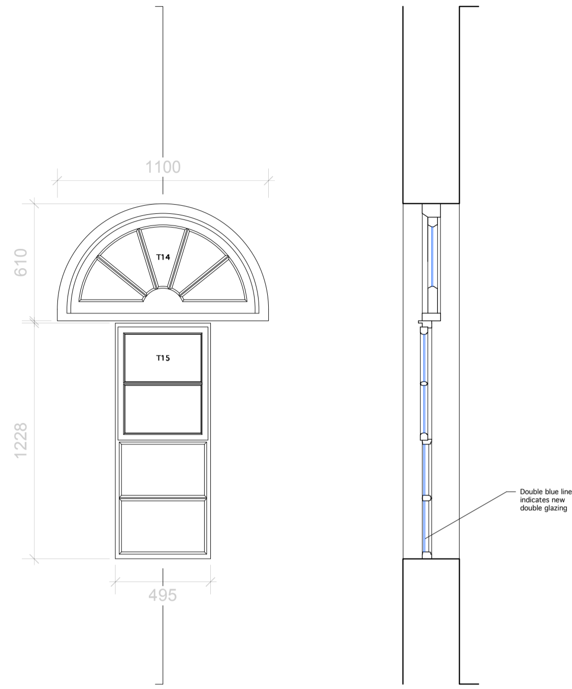
WINDOW TYPES 14, 15 Ground Floor Roger Street Extension Elevation and Section
