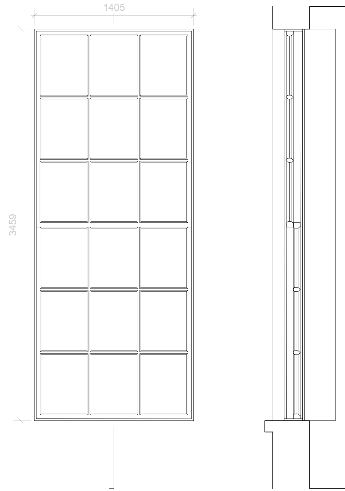
WINDOW TYPE 25 First Floor to Second Floor Stairwell Elevation and Section
