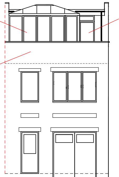
front (south east) elevation
