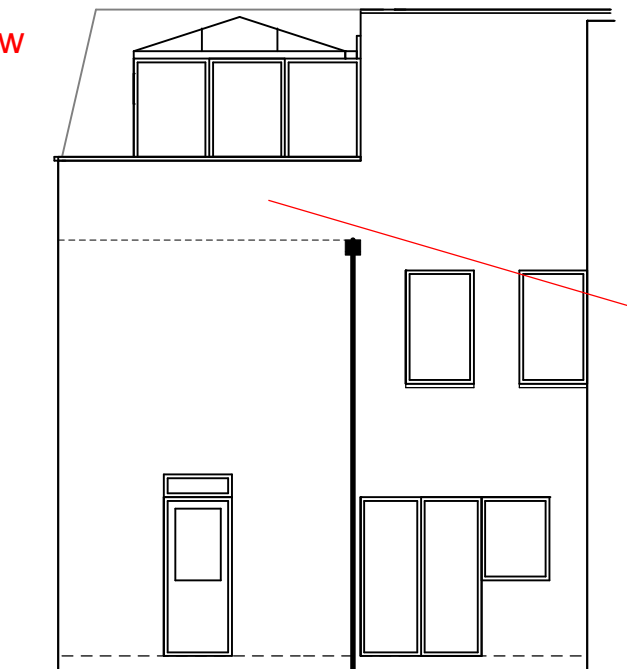
right (north east) elevation
