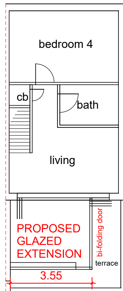
front (S/E) 2nd FLOOR LAYOUT
