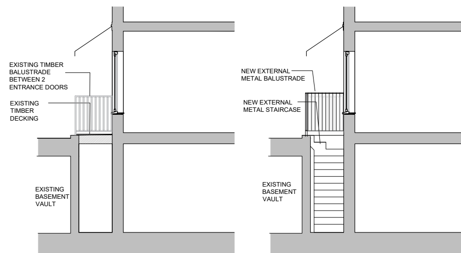
1:100 EXISTING AA SECTION
