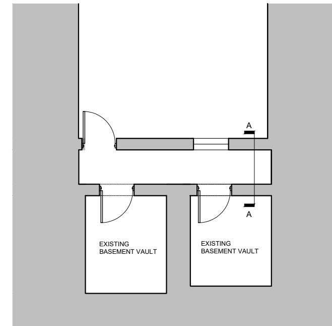
1:100 EXISTING BASEMENT PLAN
