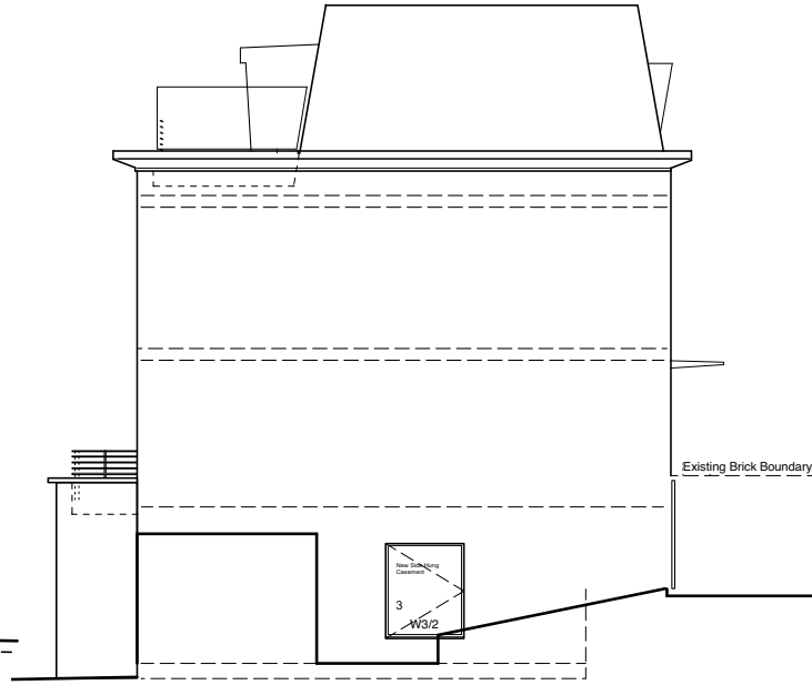
Proposed South Facing Elevation
