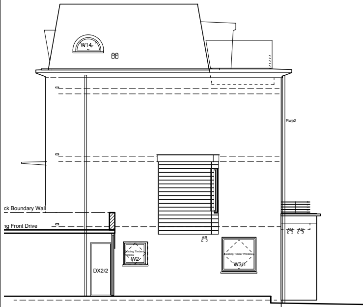
Existing North Facing Elevation
