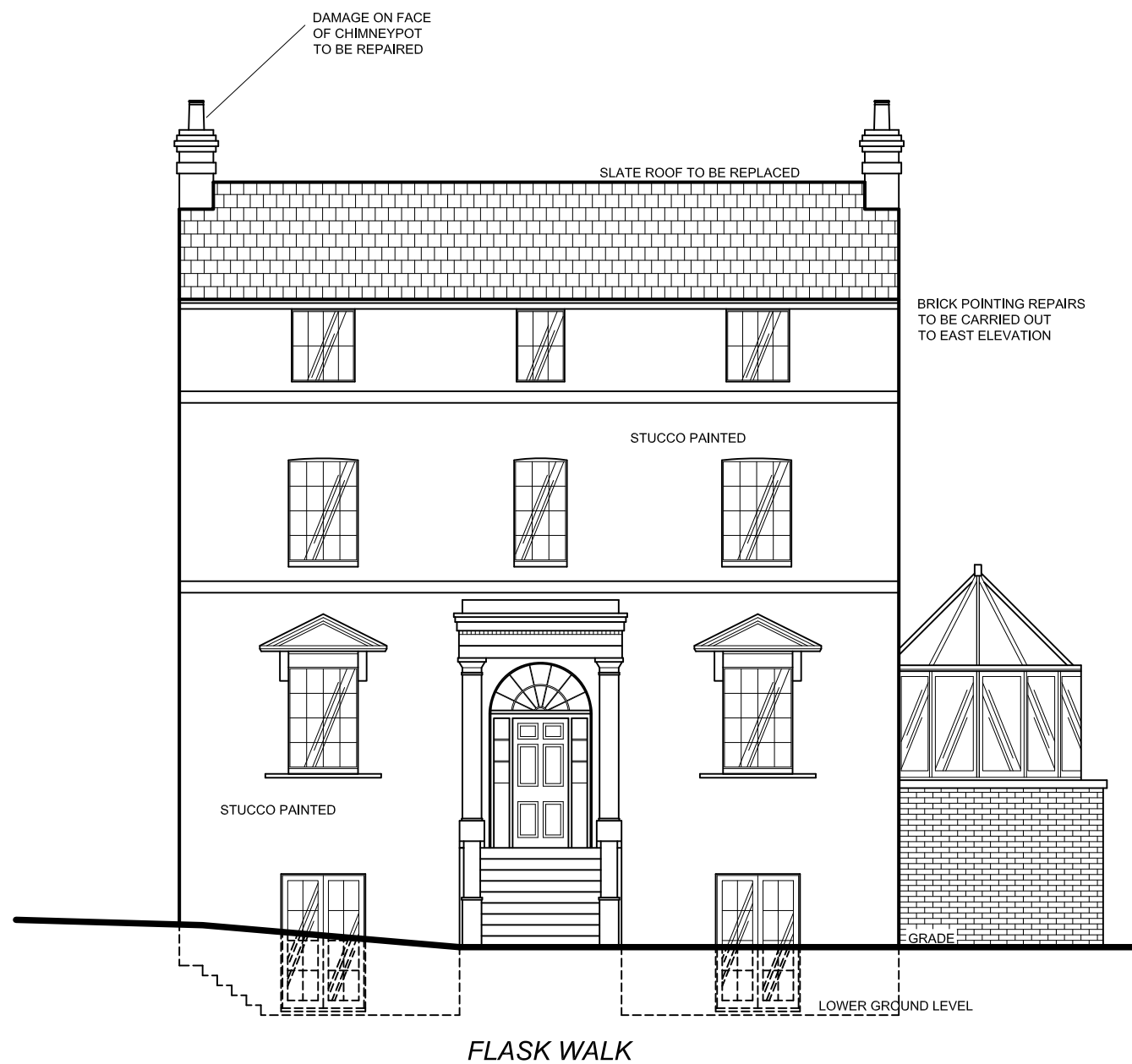
SOUTH ELEVATION
