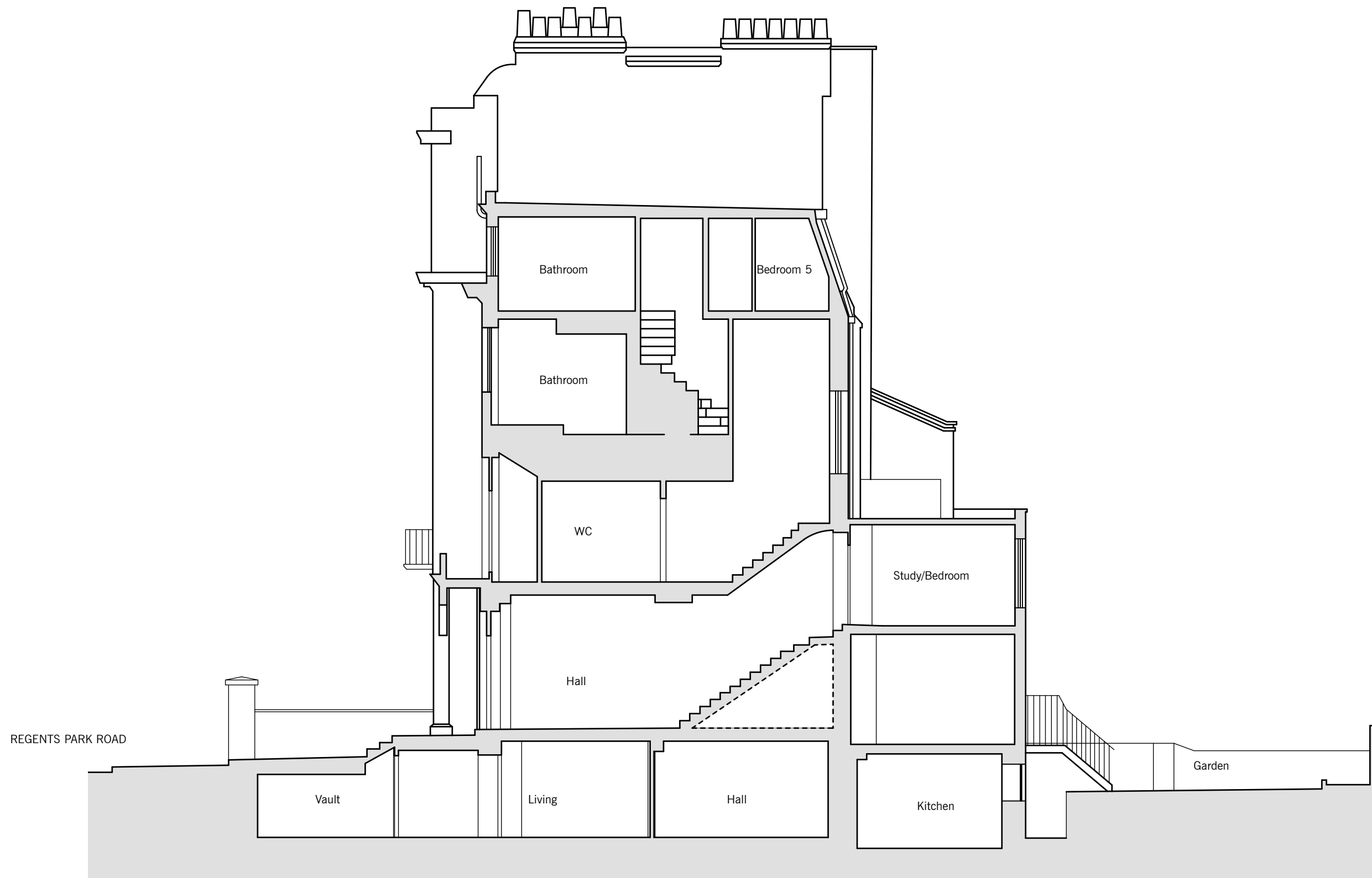
1. EXISTING SECTION AA
