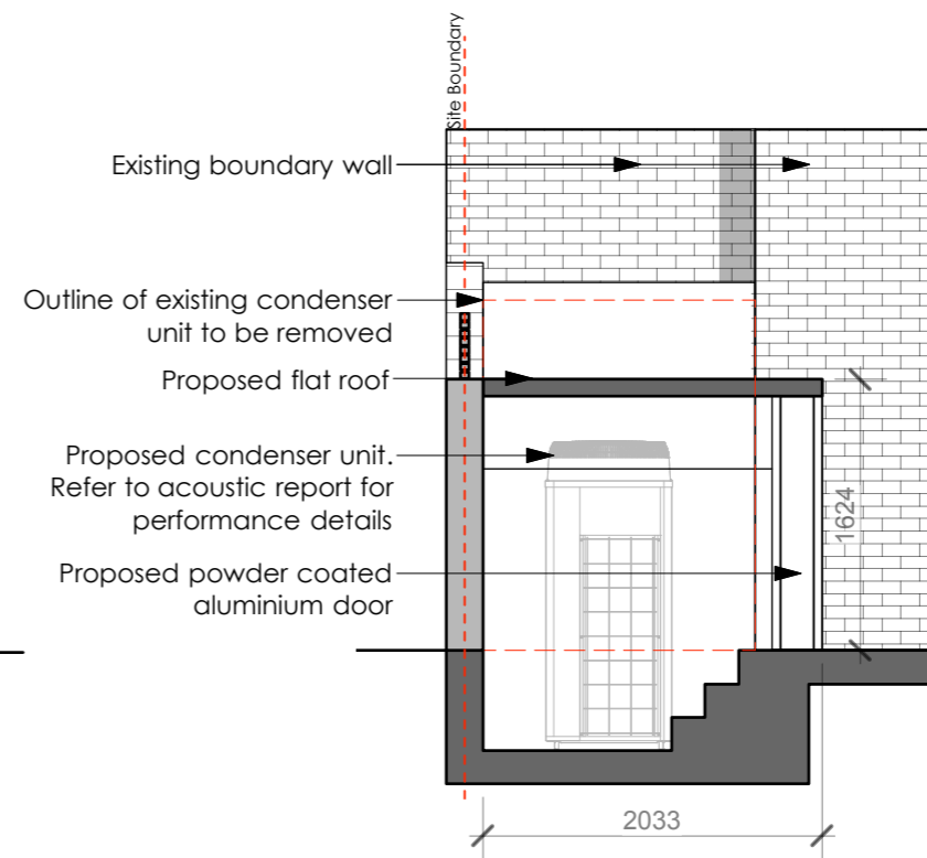
4 Proposed Section BB 1:50 @ A3
