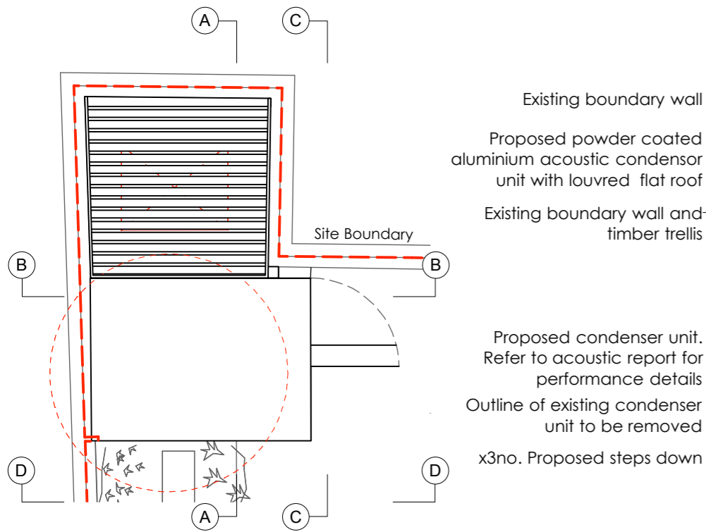
6 Key Plan @ H/L 1:50 @ A3
