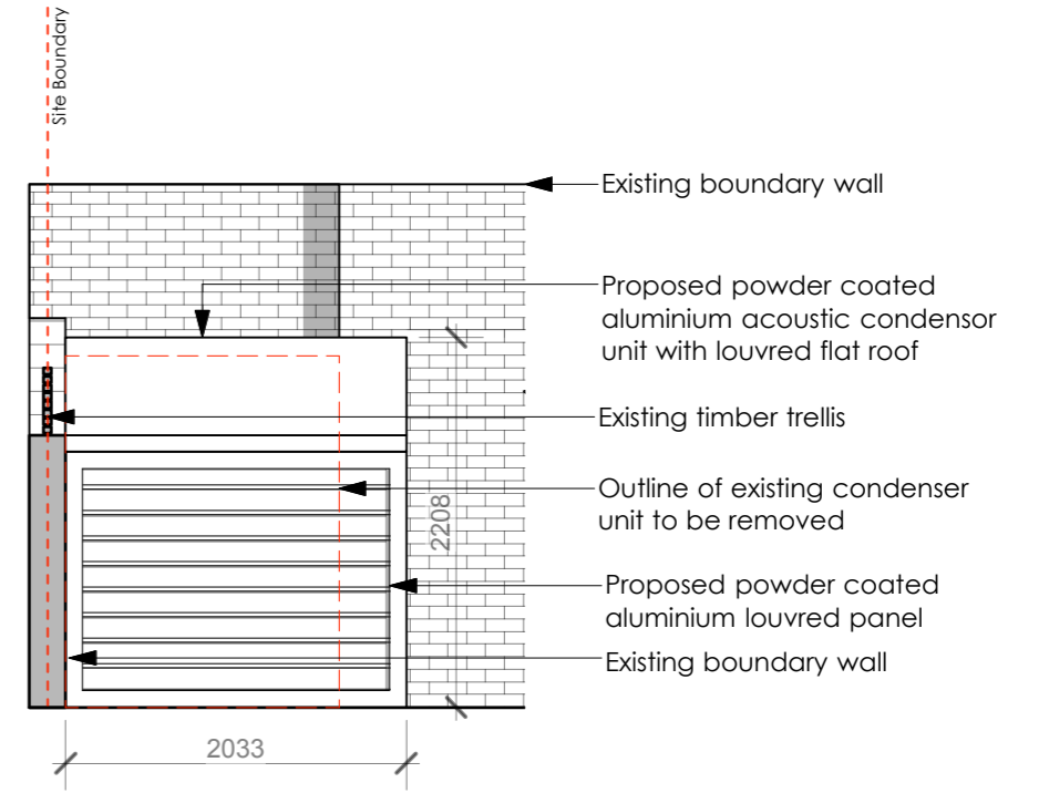
2 Proposed Elevation DD 1:50 @ A3
