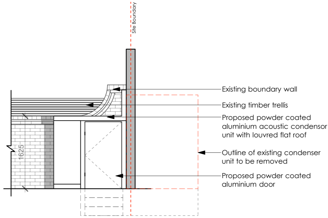
1 Proposed Elevation CC 1:50 @ A3
