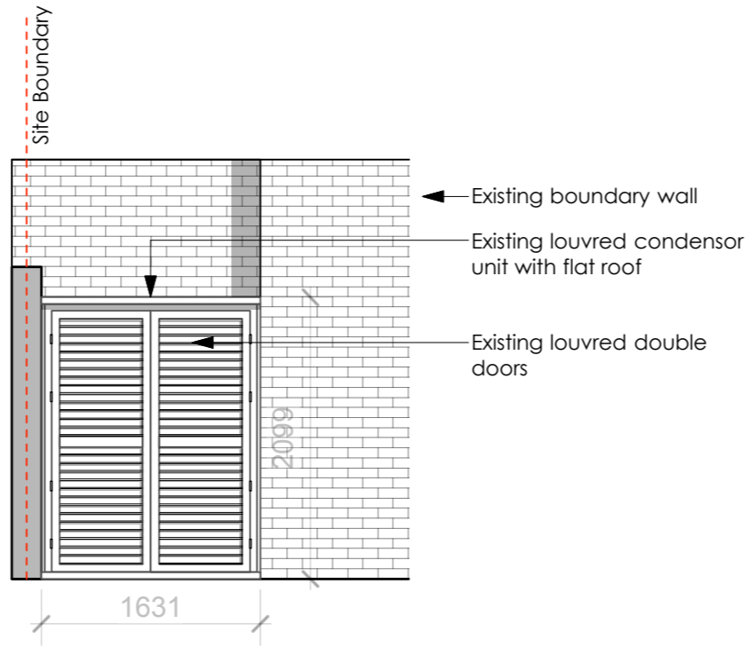
1 Existing Elevation CC
