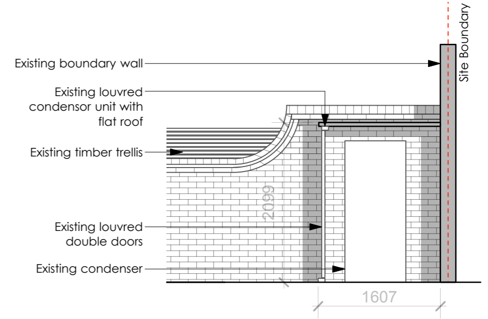
2 Existing Section AA
