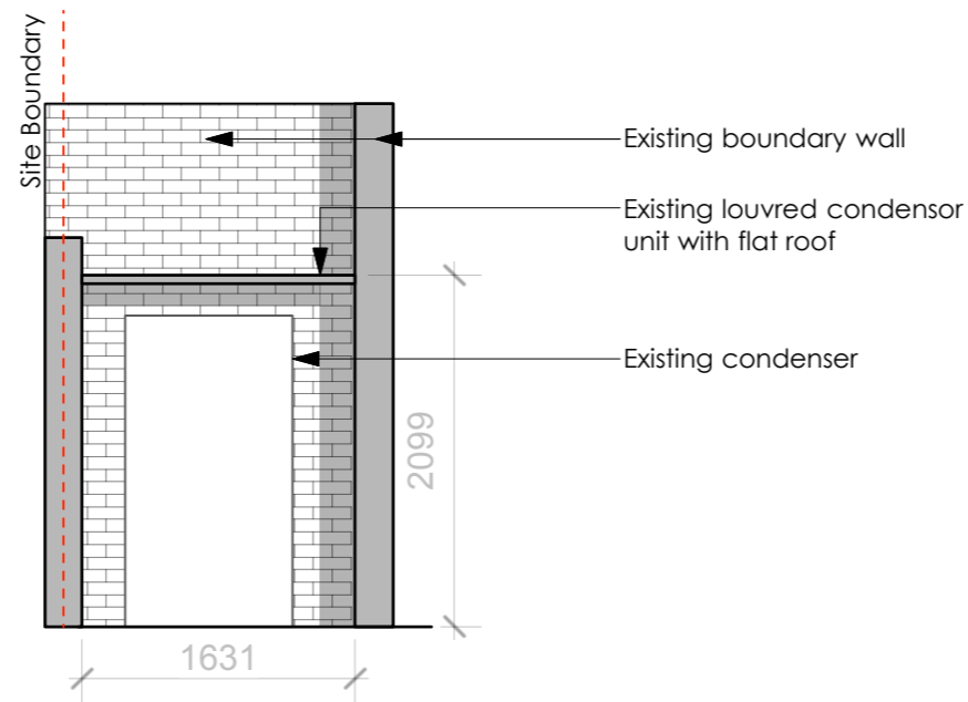
3 Existing Section BB
