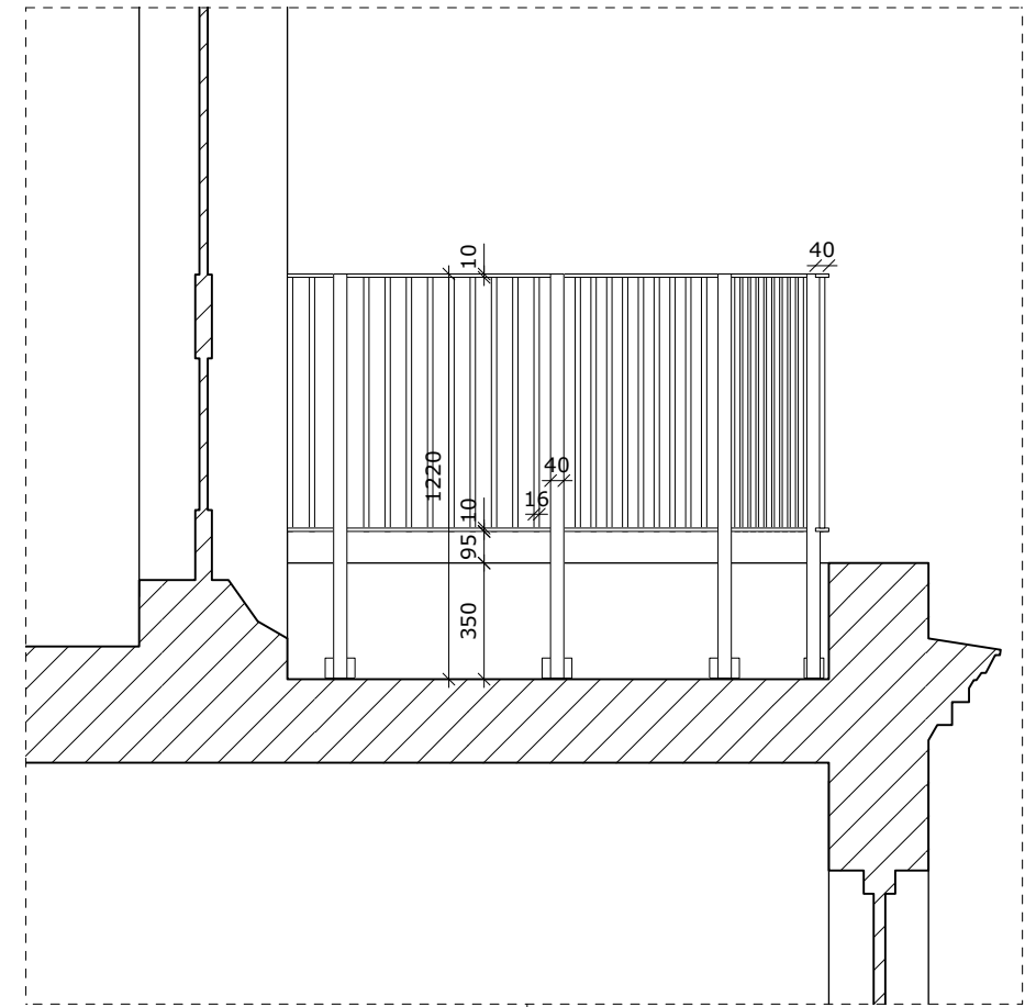
3 Detail Section 1:25
