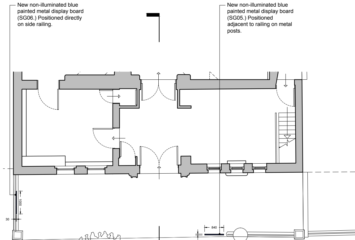
PROPOSED PLAN 1:100 @ A3
