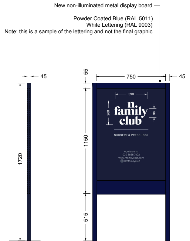
DISPLAY BOARD (SG05) ELEVATION & SECTION DETAILS 1:25 @ A3
