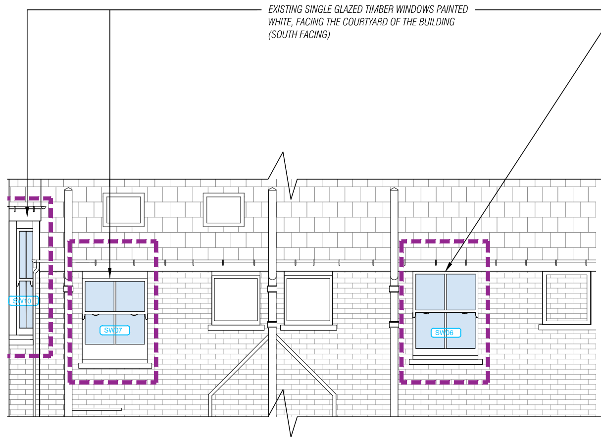
01 | EXISTING SOUTH ELEVATION 'A'_THE PRYORS (COURTYARD) Scale: 1/50 @ A3
