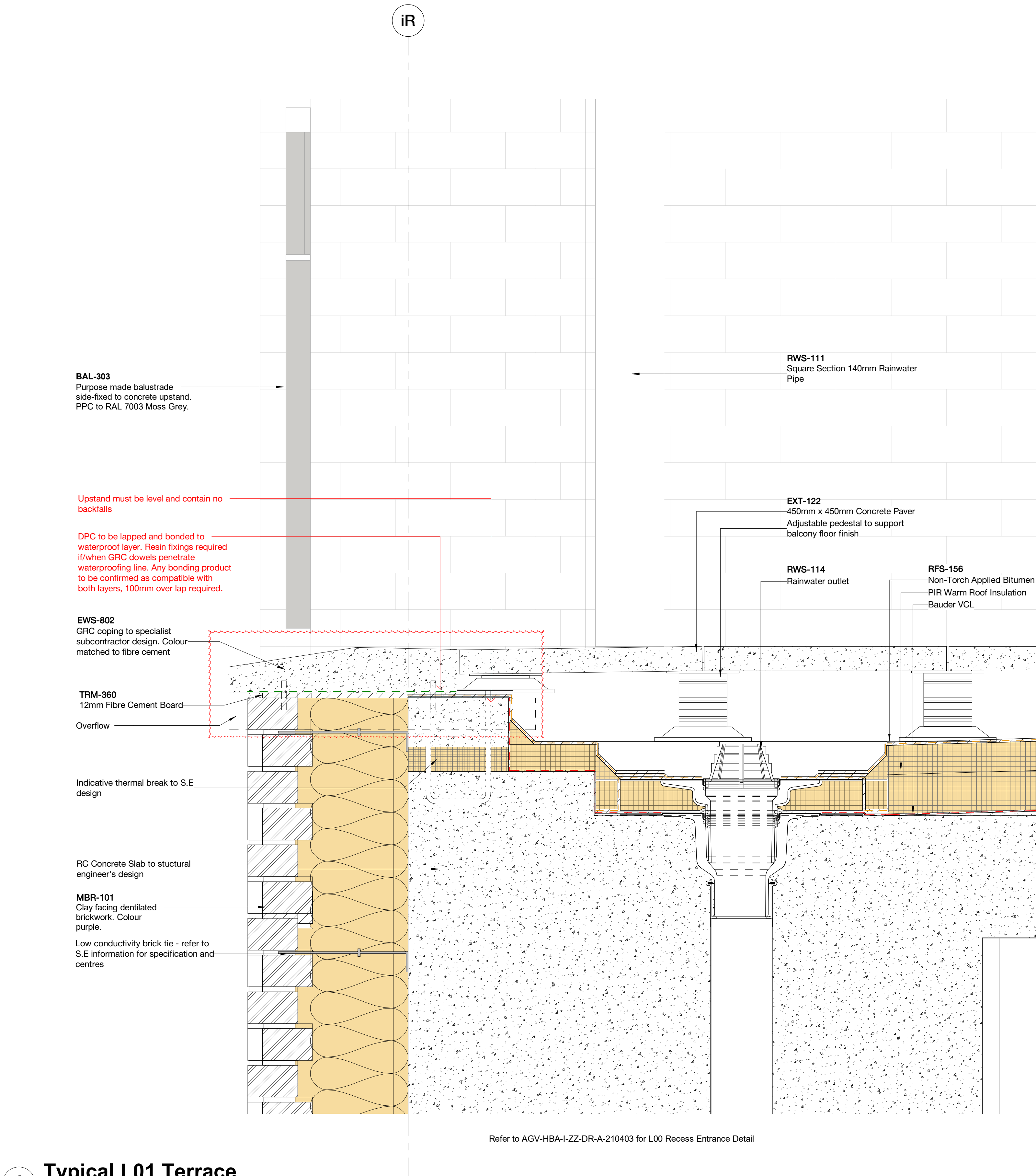
1 Typical L01 Terrace 1 : 5
