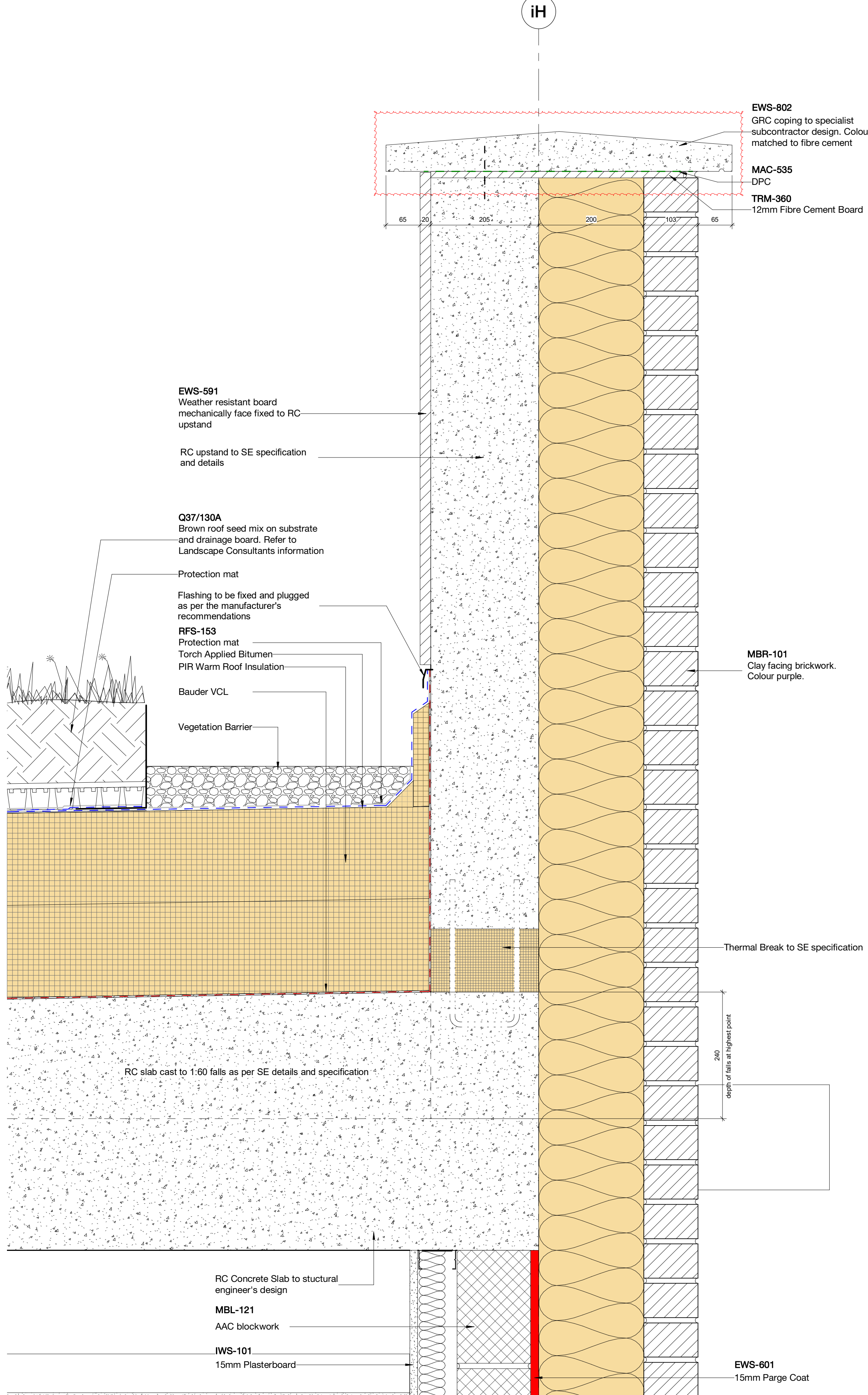
2 LRF Parapet - High Point 1:5
