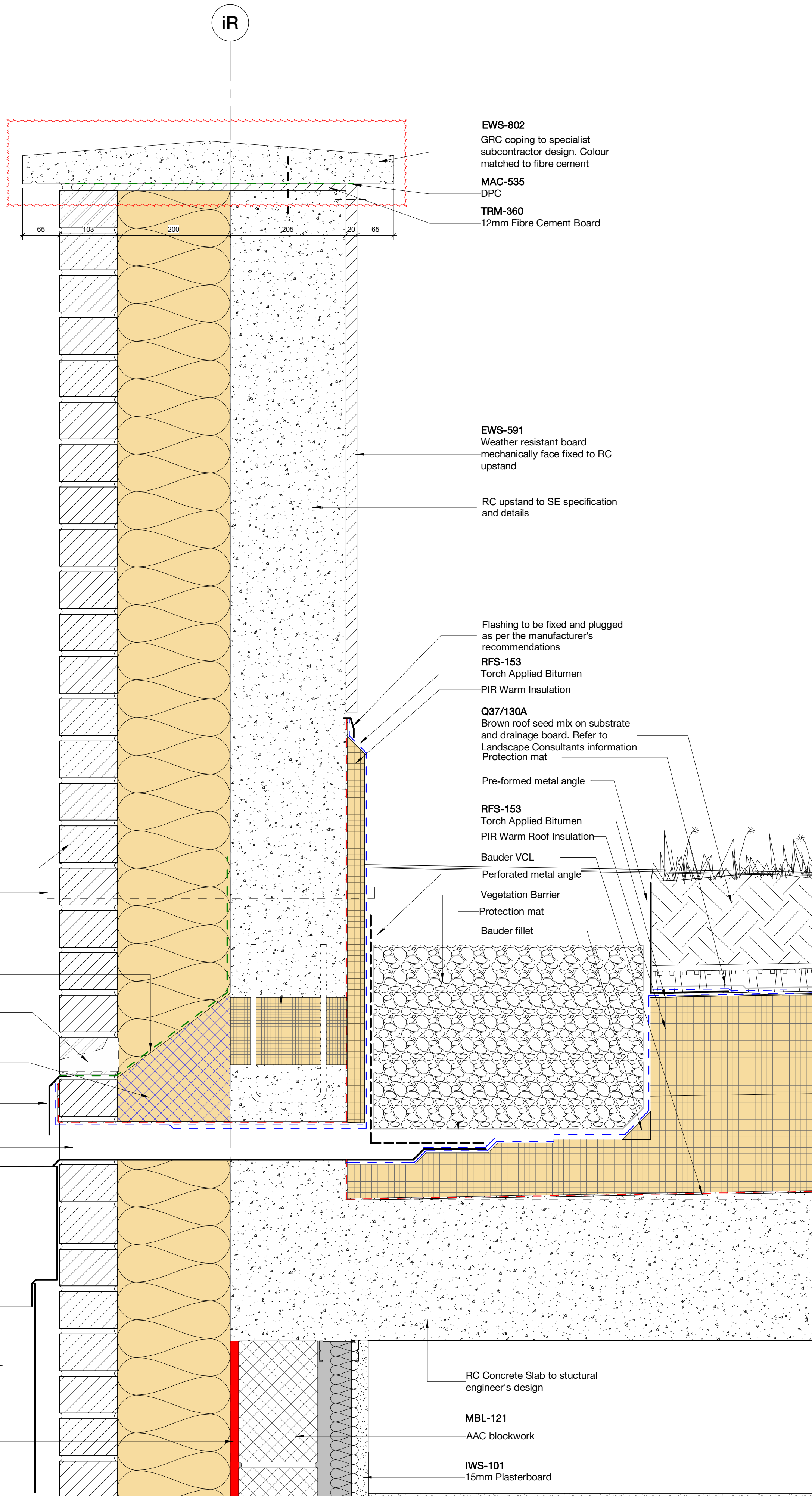
1 LRF Parapet - Low Point & Hopper Head Detail 1:5
