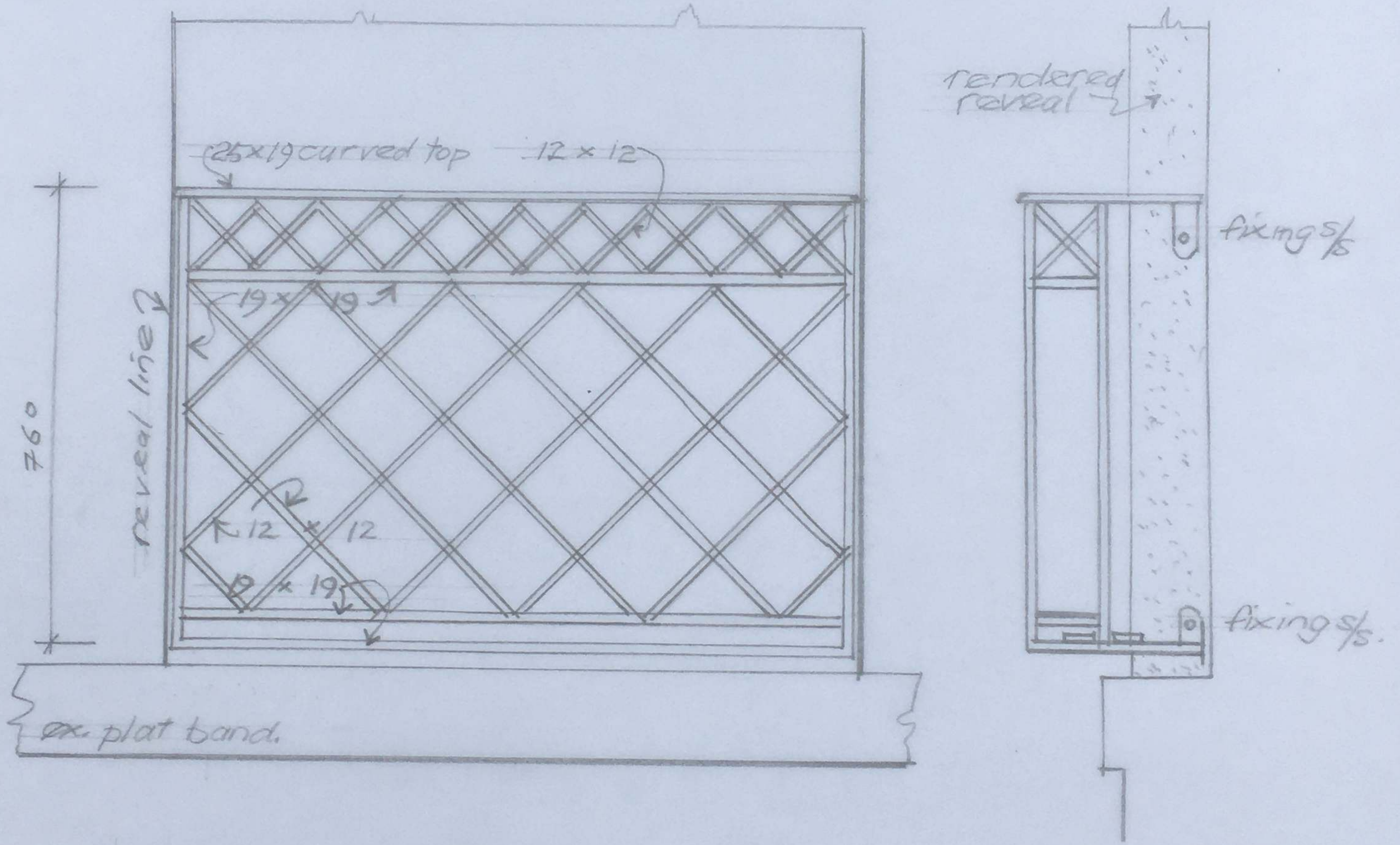
Window Boxes. First Floor. 1:10 @ A3.
