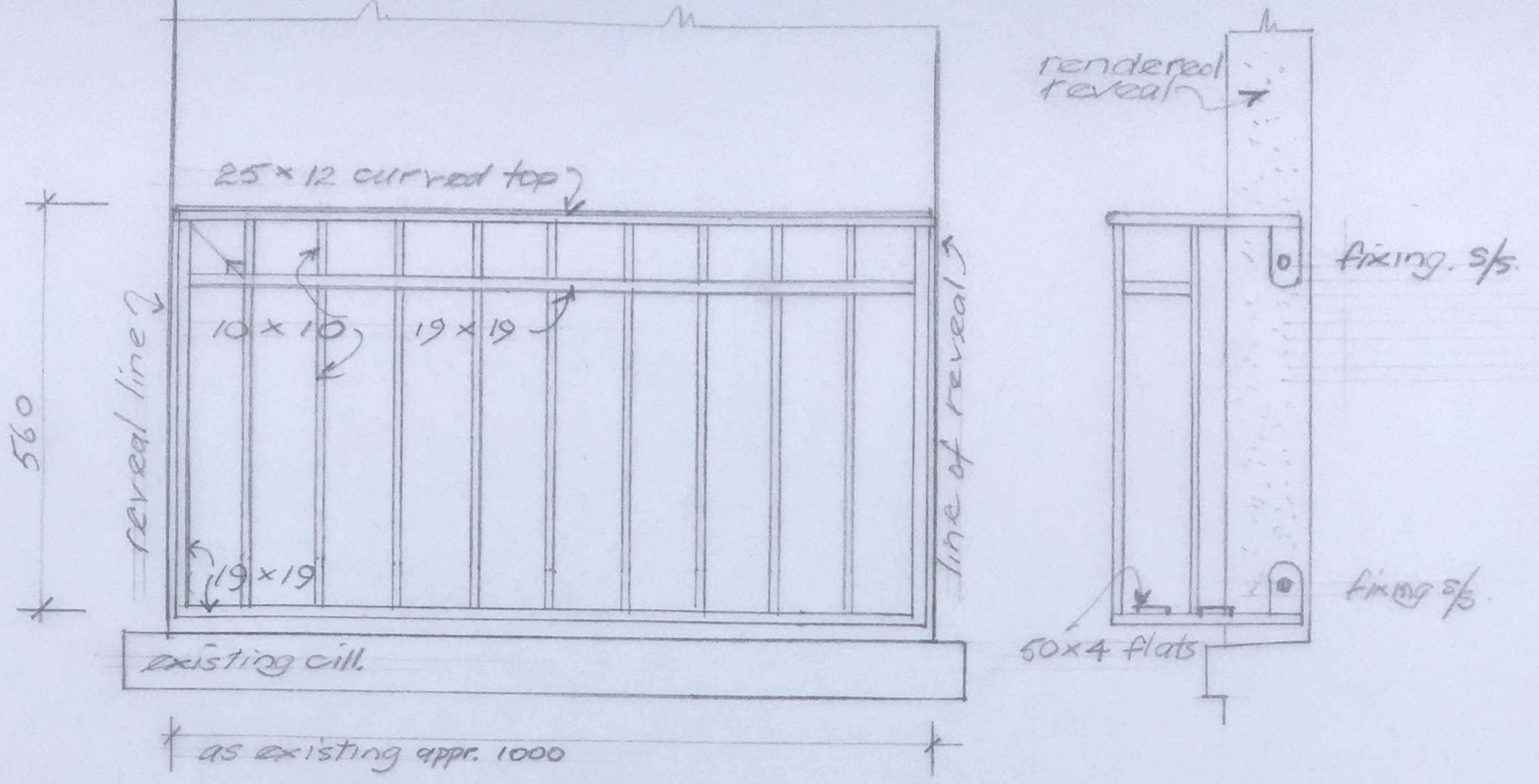
Window Boxes. Second Floor. 1:10 (at A3)
