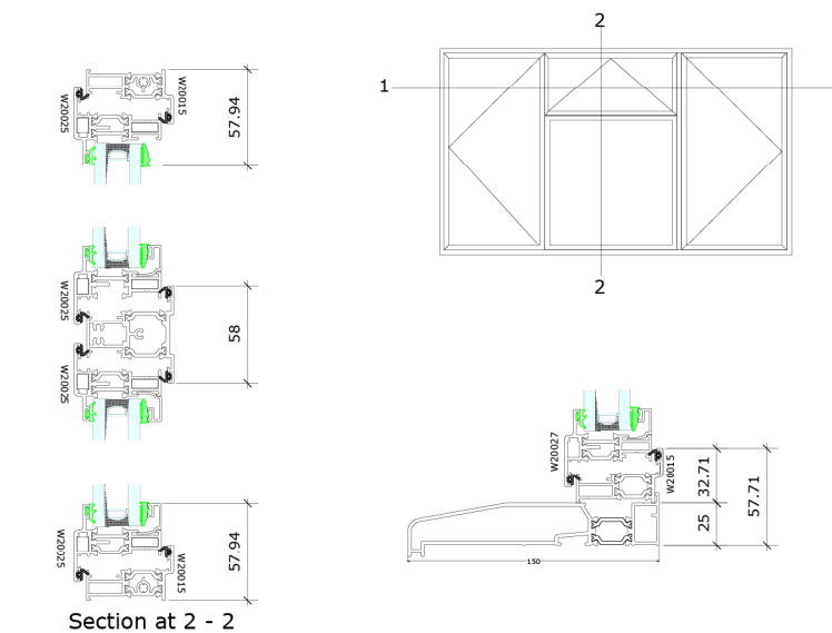
Section at 2 - 2
