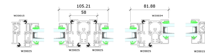
Section at 1 - 1
