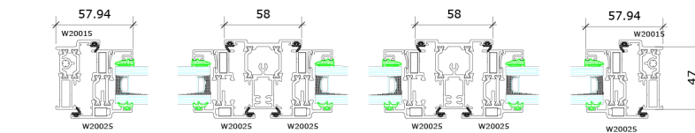
Section at 1 - 1
