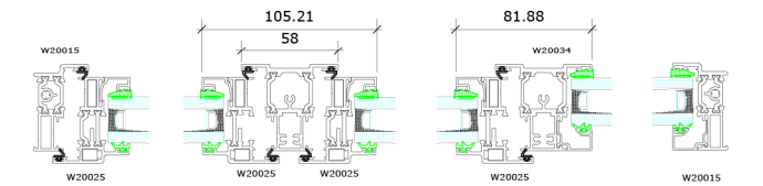
Section at 1 - 1
