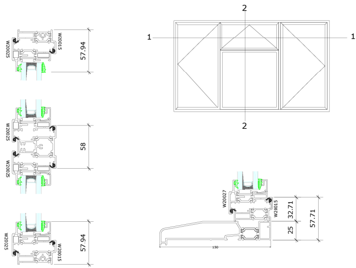
Section at 2 - 2
