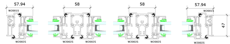
Section at 2 - 2
