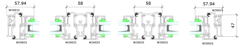
Section at 1 - 1
