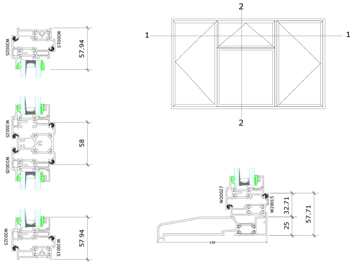
Section at 2 - 2
