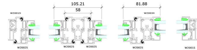
Section at 1 - 1
