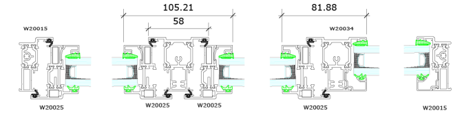
Section at 1 - 1
