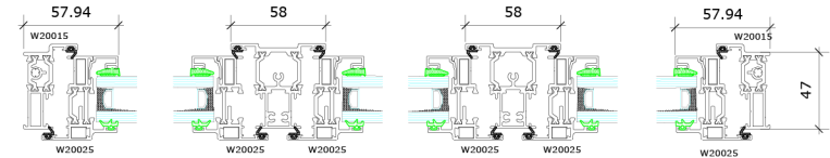
Section at 1 - 1
