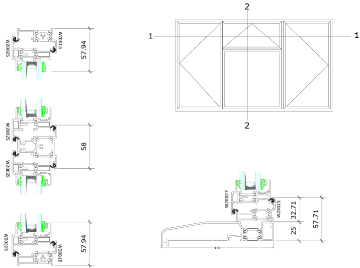
Section at 2 - 2
