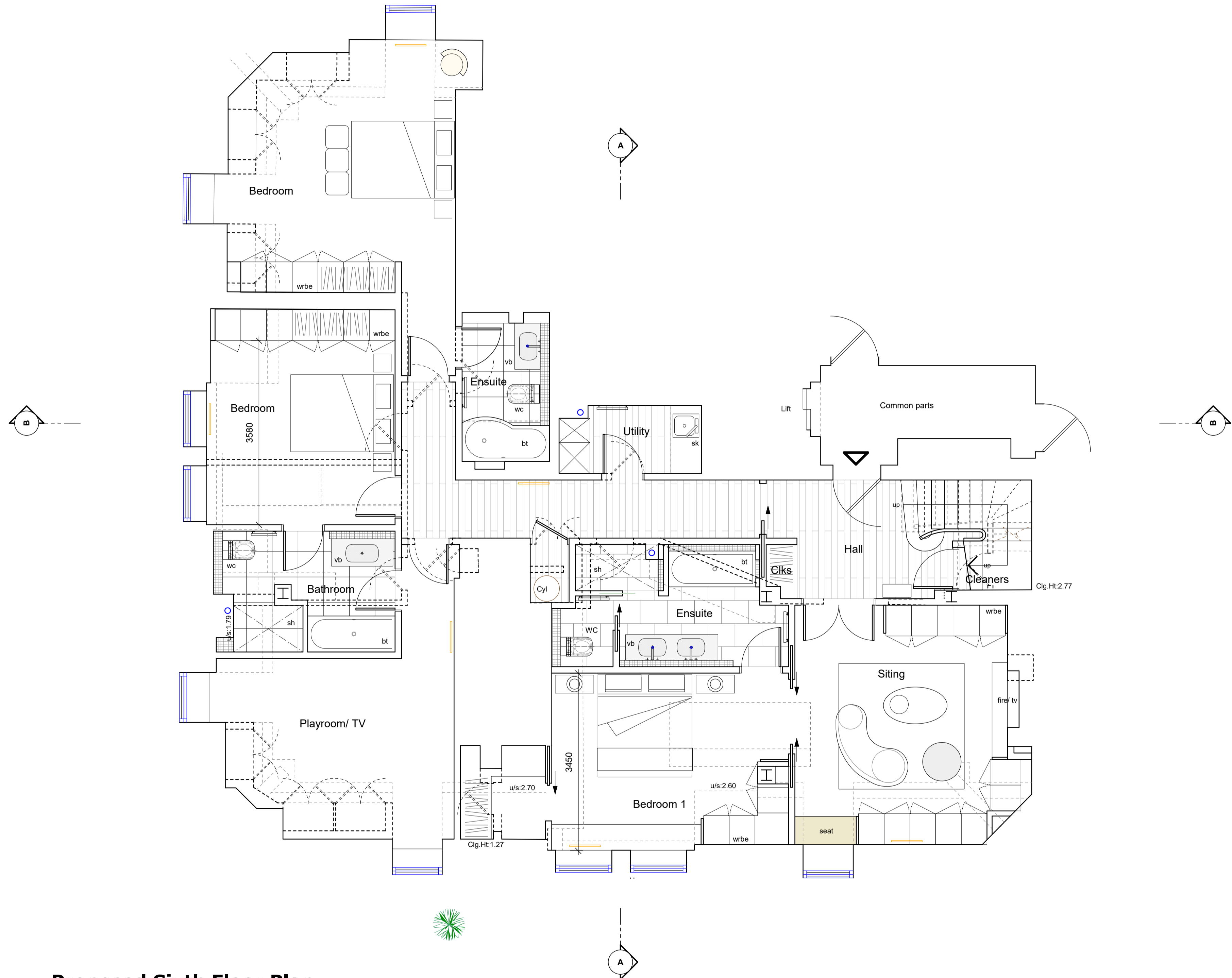
Proposed Sixth Floor Plan (1:50 @ A1)
