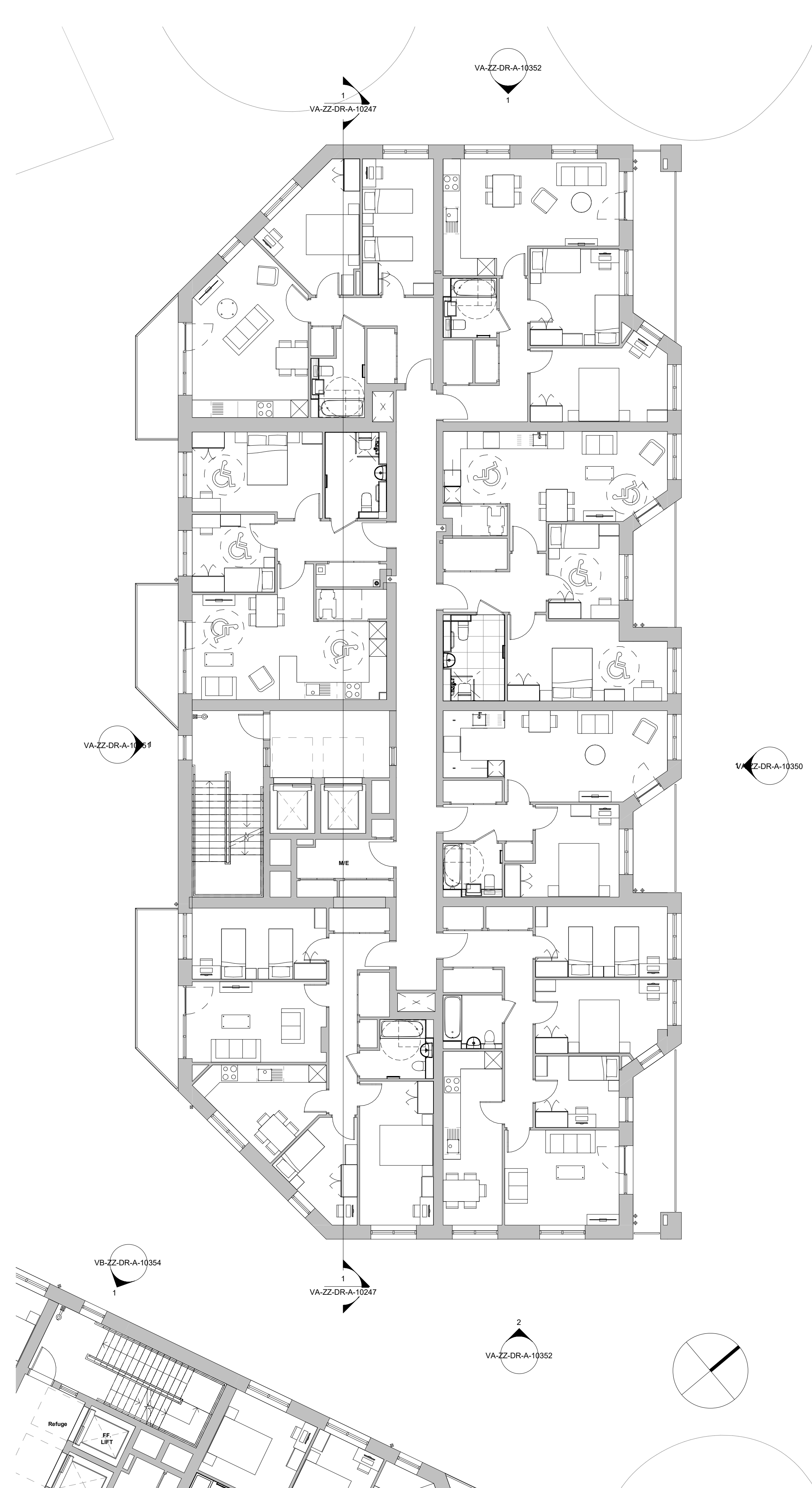
2 AA.01 - First Floor - Fifth Floor 1_100 Scale: 1:100
