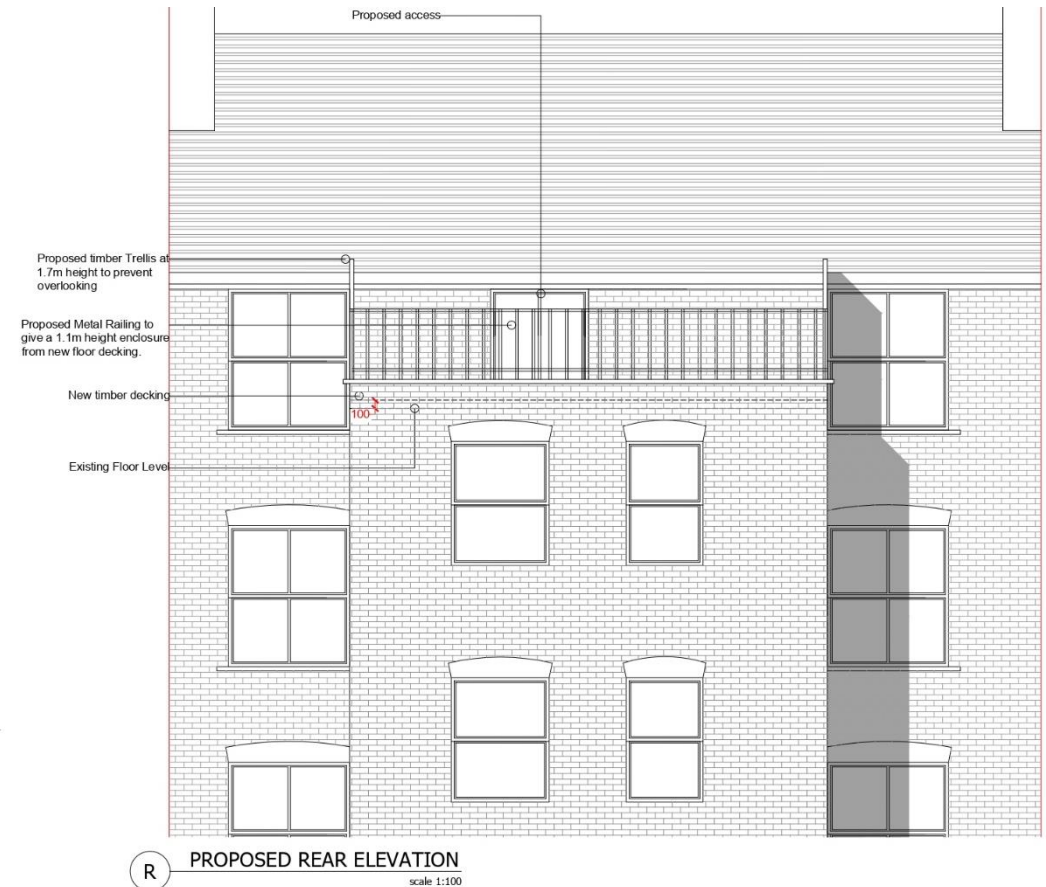
Figure 2: Proposed Rear Elevation
