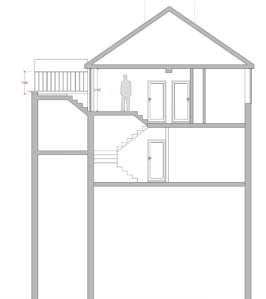
Figure 4: Proposed Section
