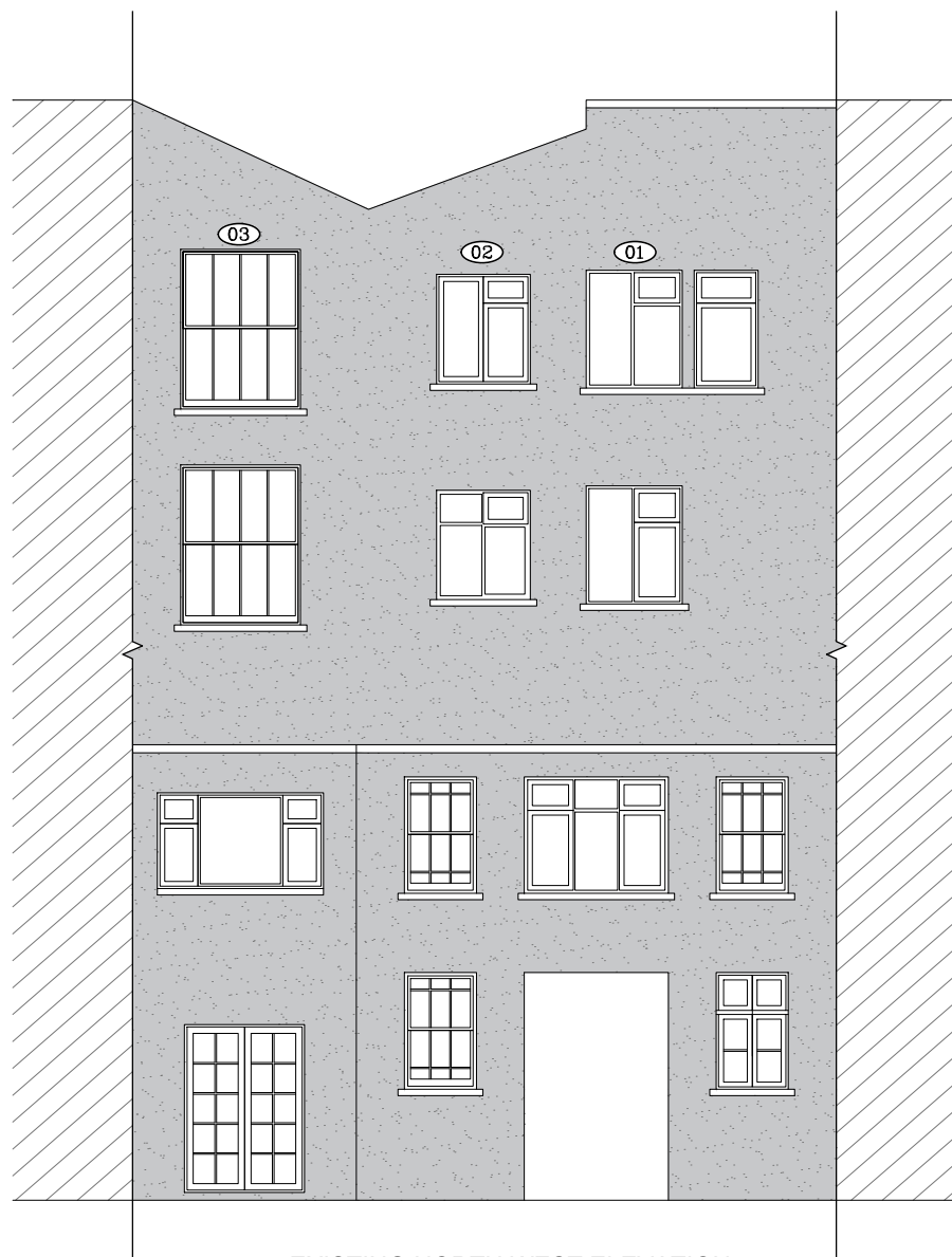
EXISTING NORTH WEST ELEVATION
