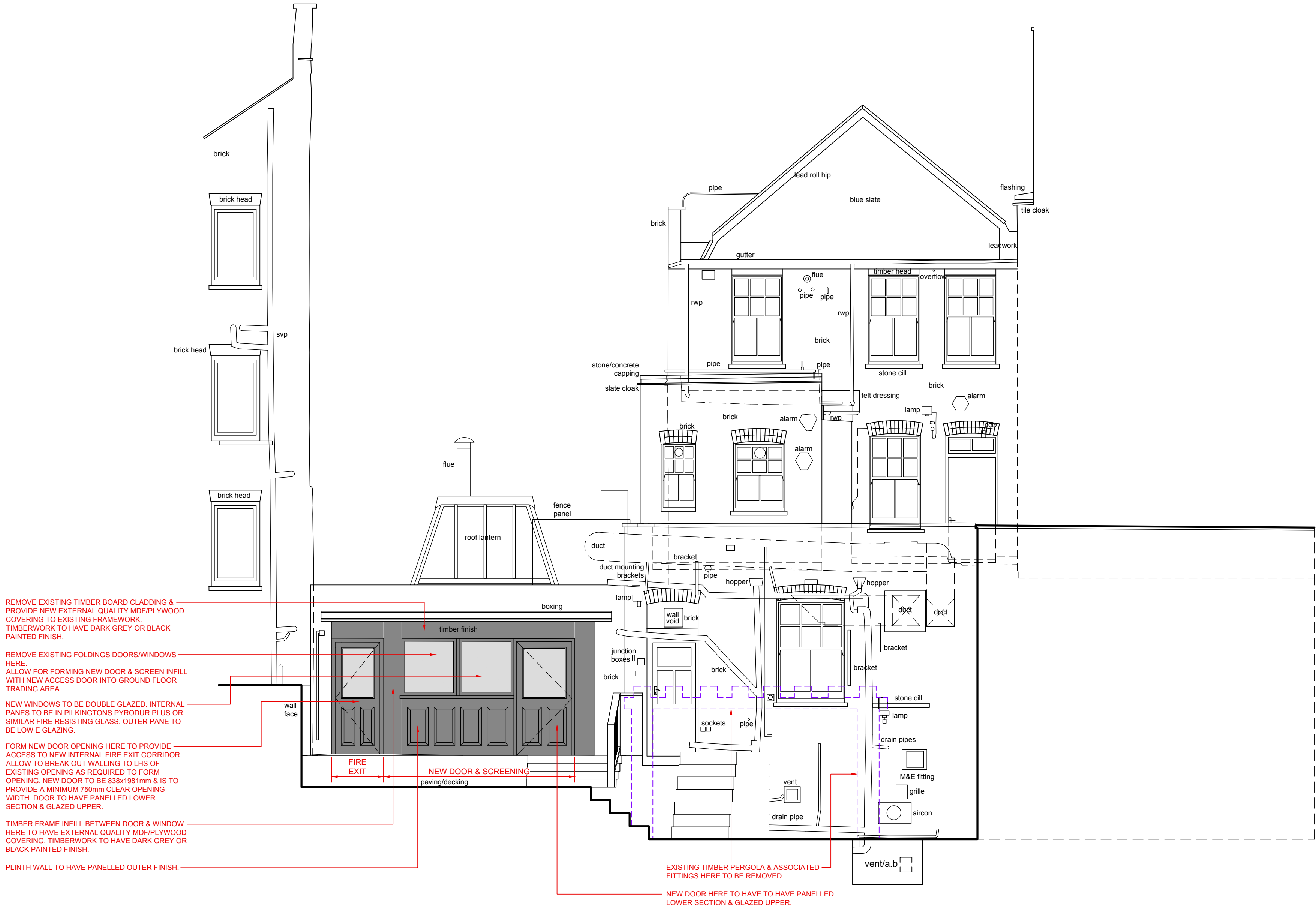
ELEVATION D-D. LOOKING TOWARDS REAR OF BUILDING SHOWING NEW DOORS & SCREENING. (NEW PERGOLA & RAILINGS OMITTED).
