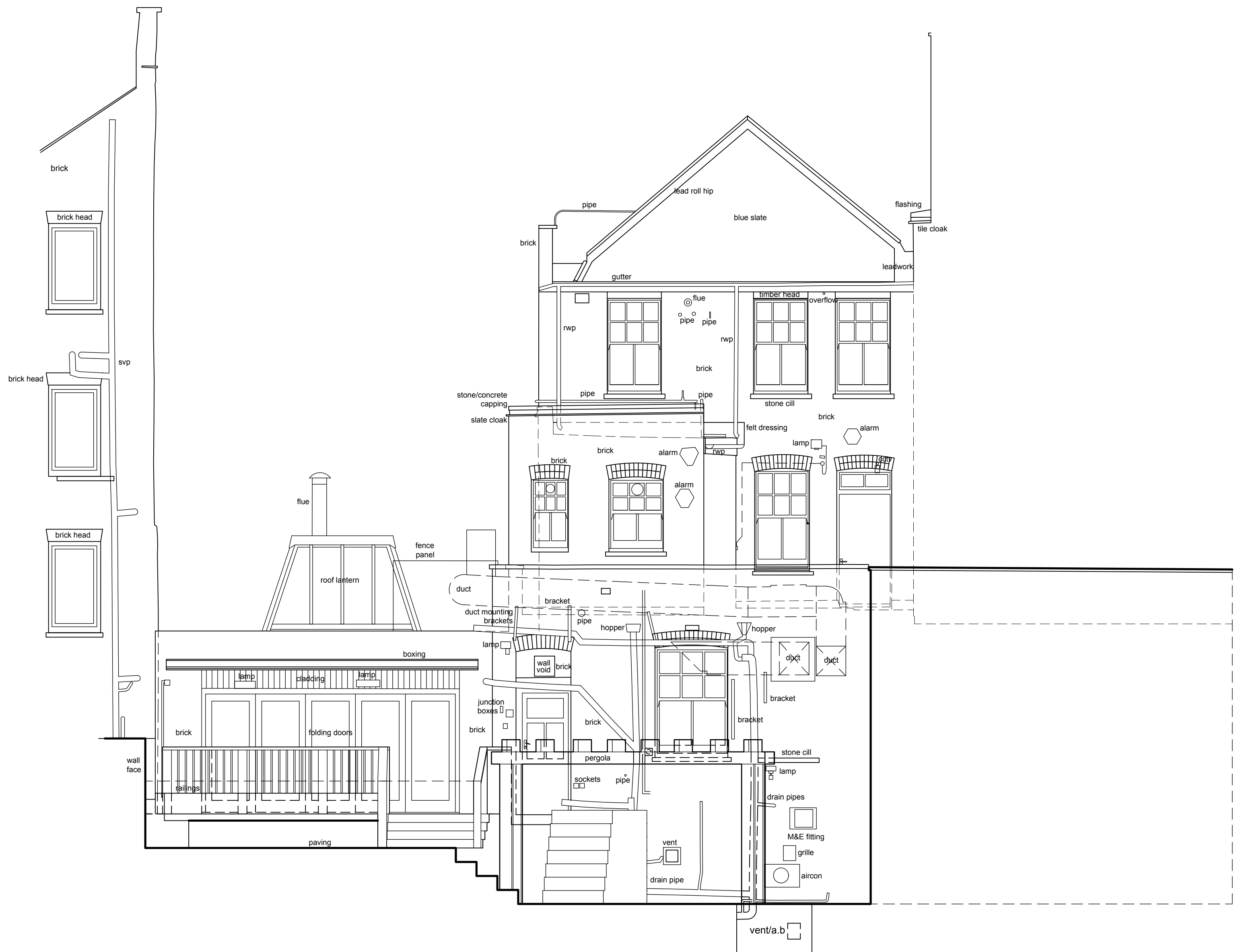
REAR (SOUTH WEST) ELEVATION.
