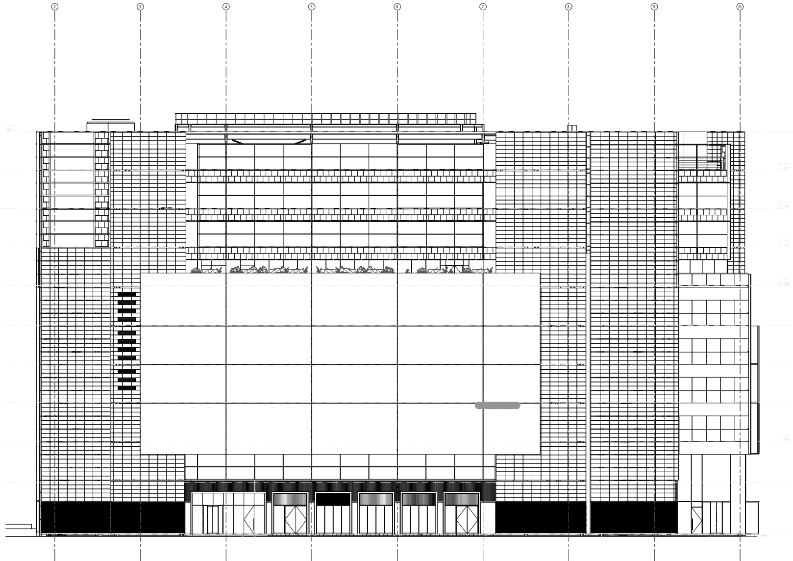
SOUTH ELEVATION
