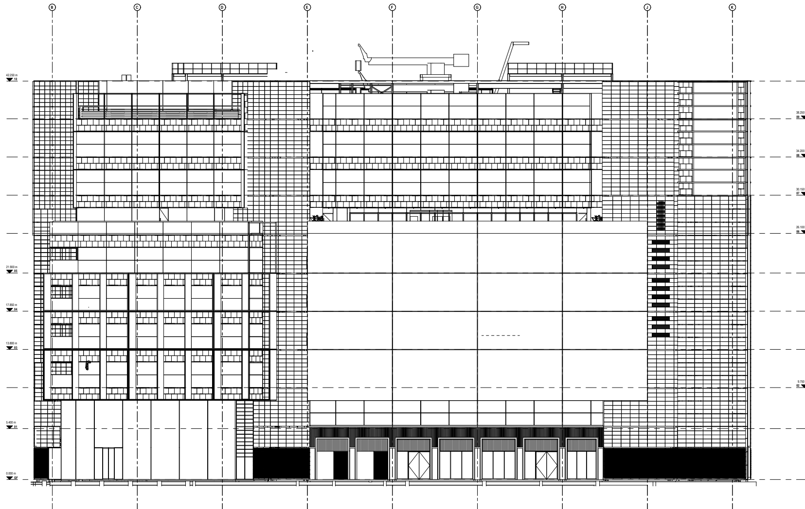
EAST ELEVATION
