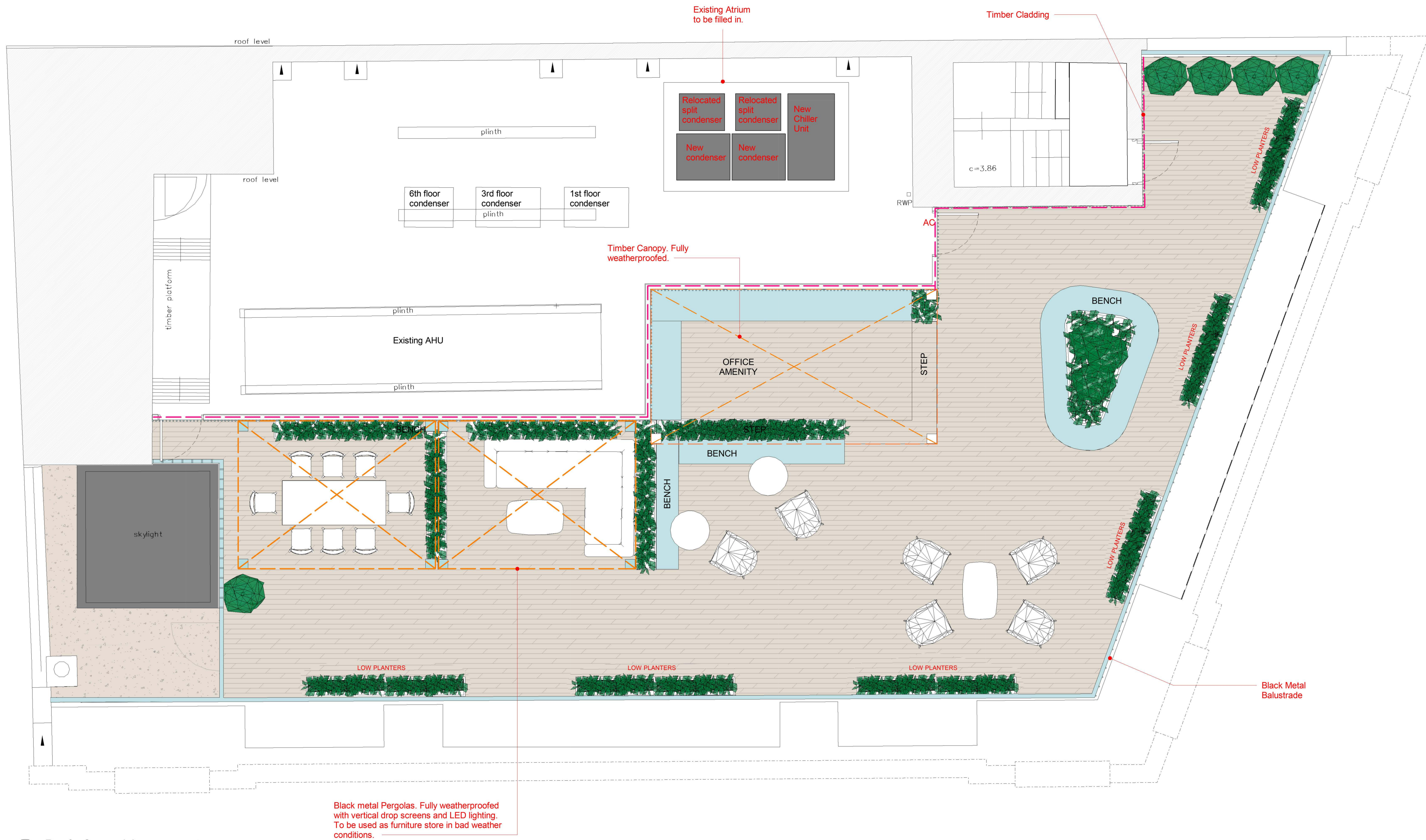
1 Roof - General Arrangement 1 : 50
