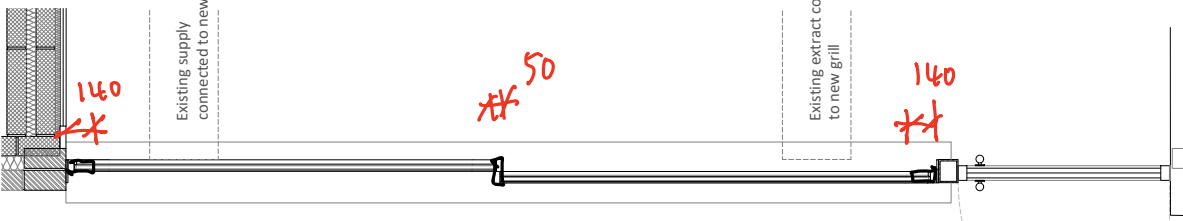
03 Window Detail Plan
