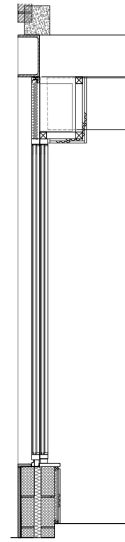
02 Window Detail Section
