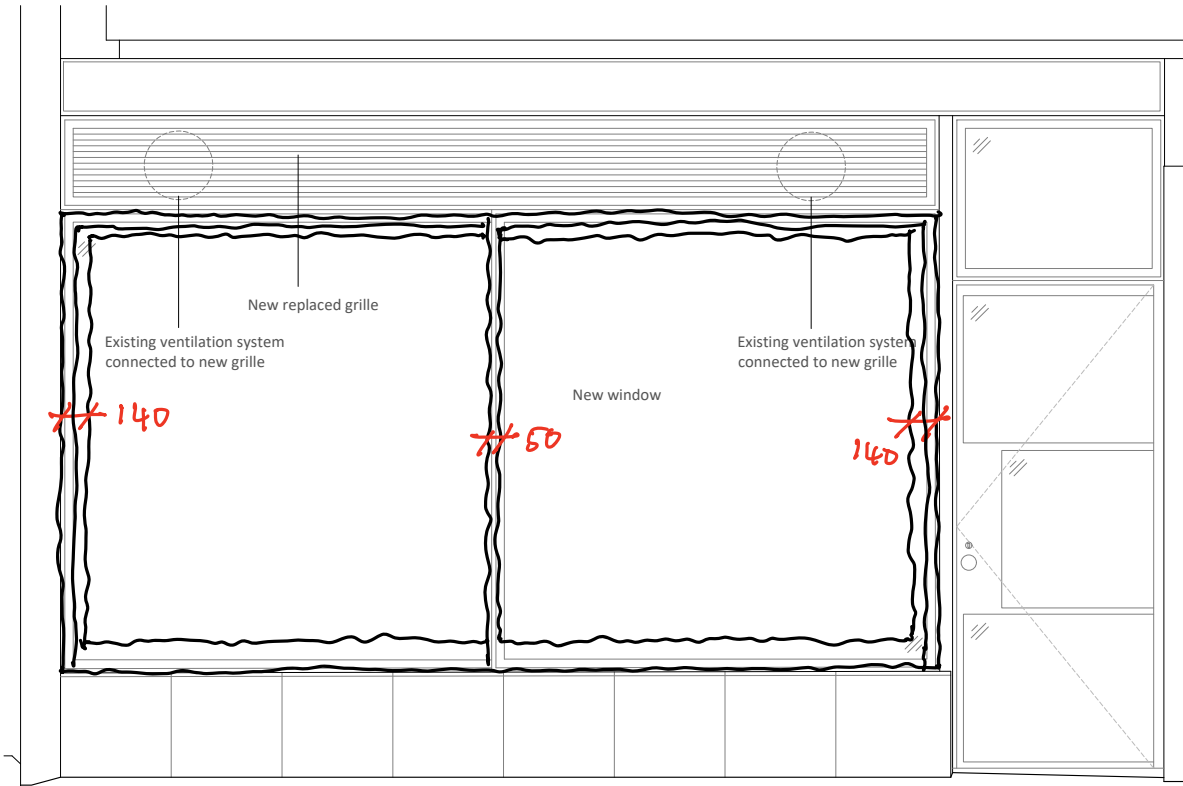
01 Window Detail Elevation
