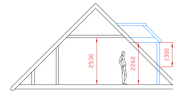
Proposed Section
