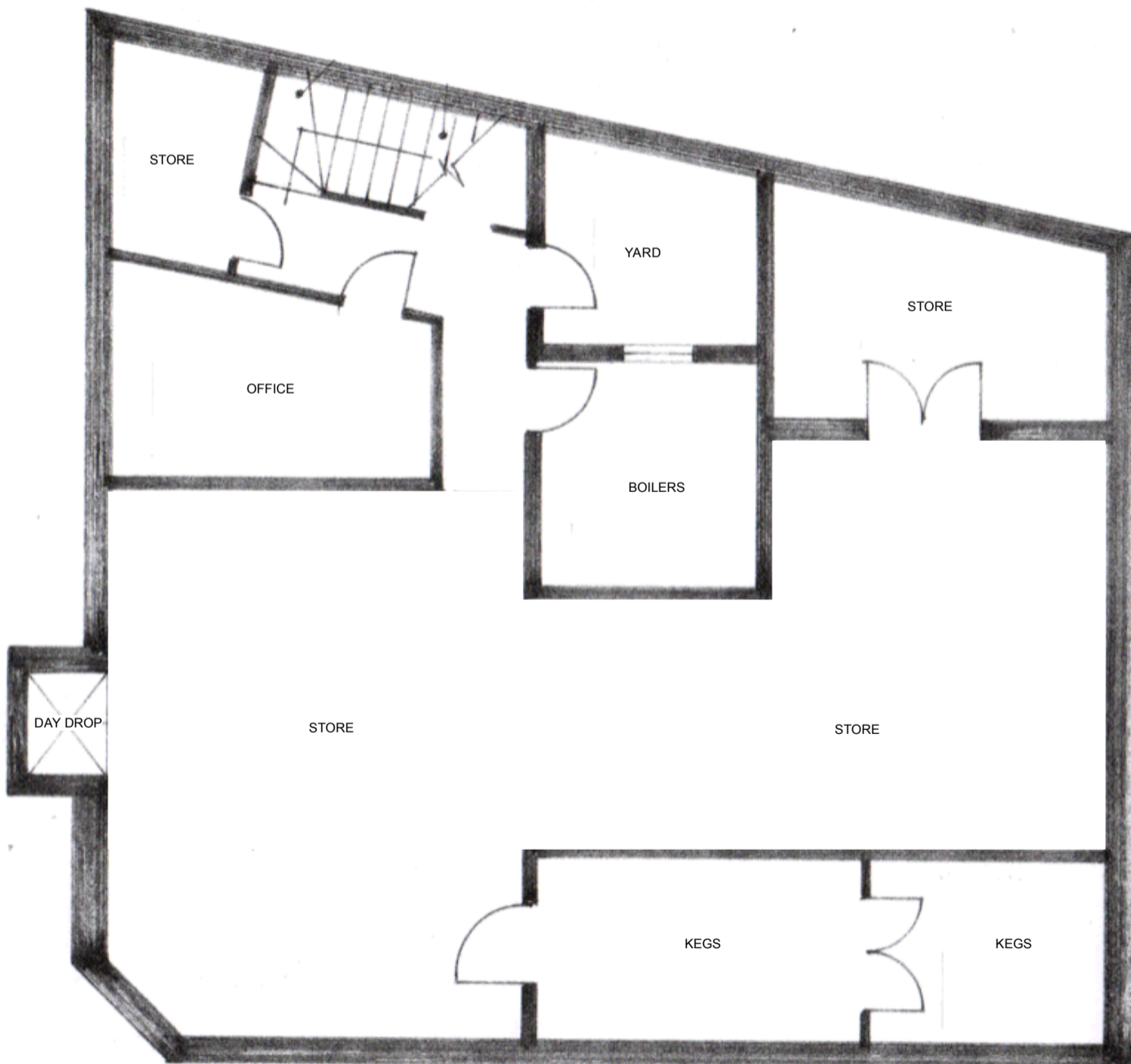
BASEMENT PLAN
