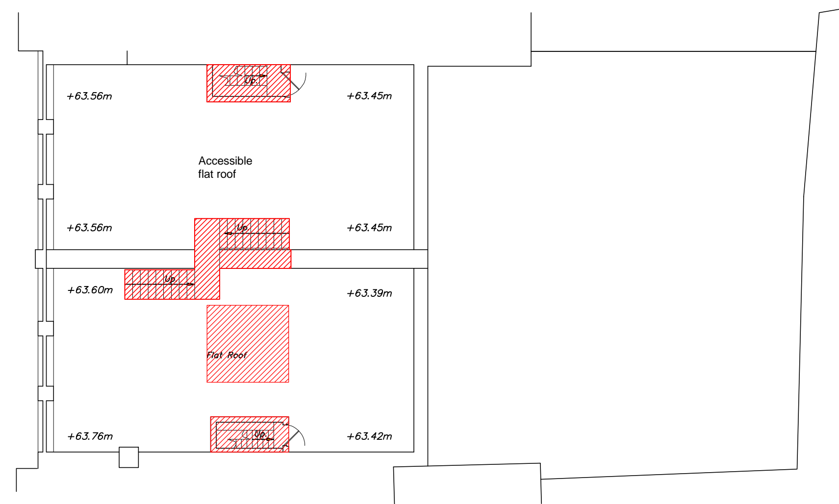
Existing Roof Plan & Demolitions Scale 1:100
