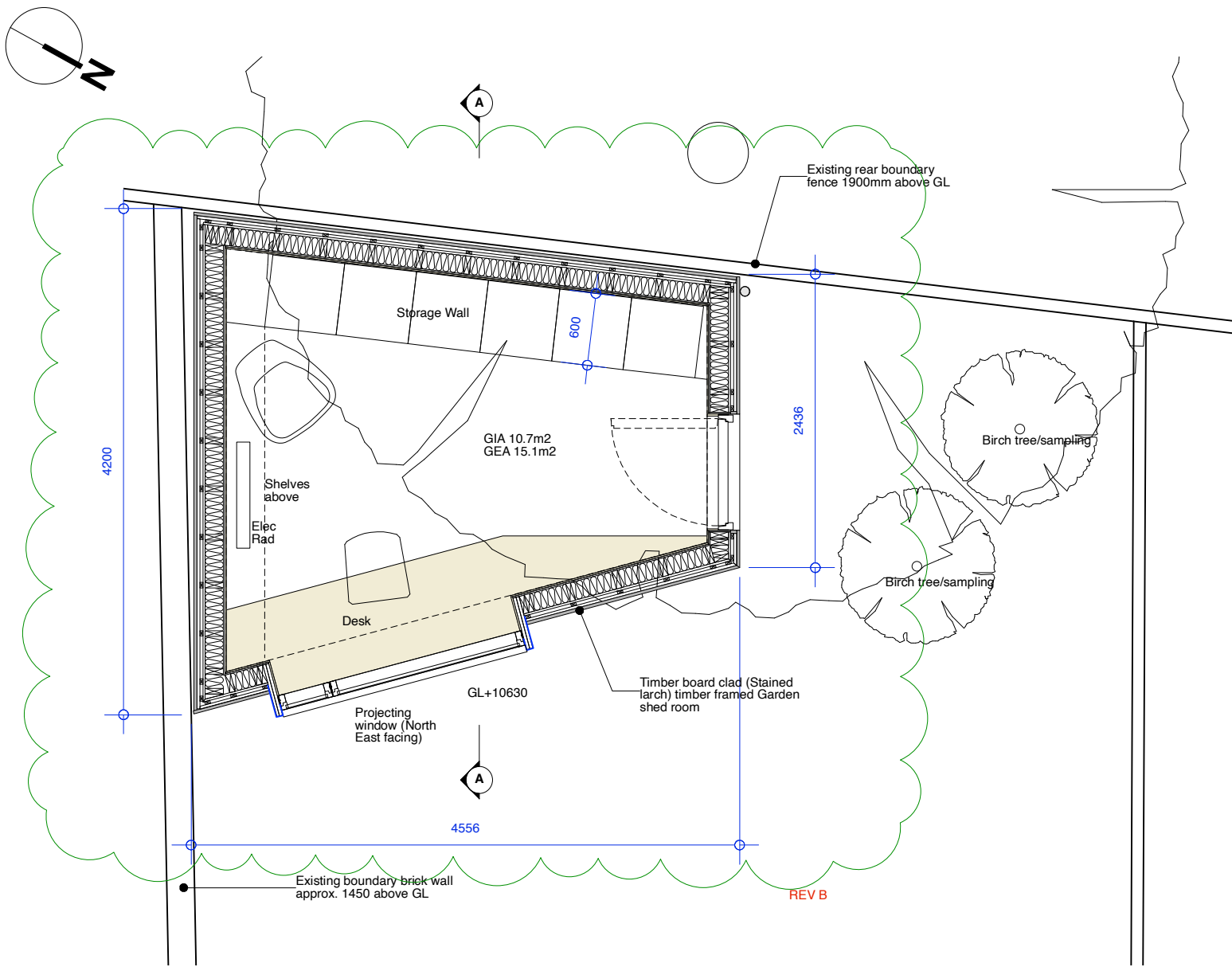
1 Proposed Garden Room Floor Plan Scale: 1:50
