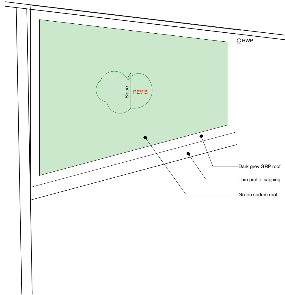
2 Proposed Garden Room Roof Plan Scale: 1:50
