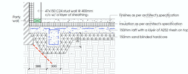
4 Garden room foundation detail
