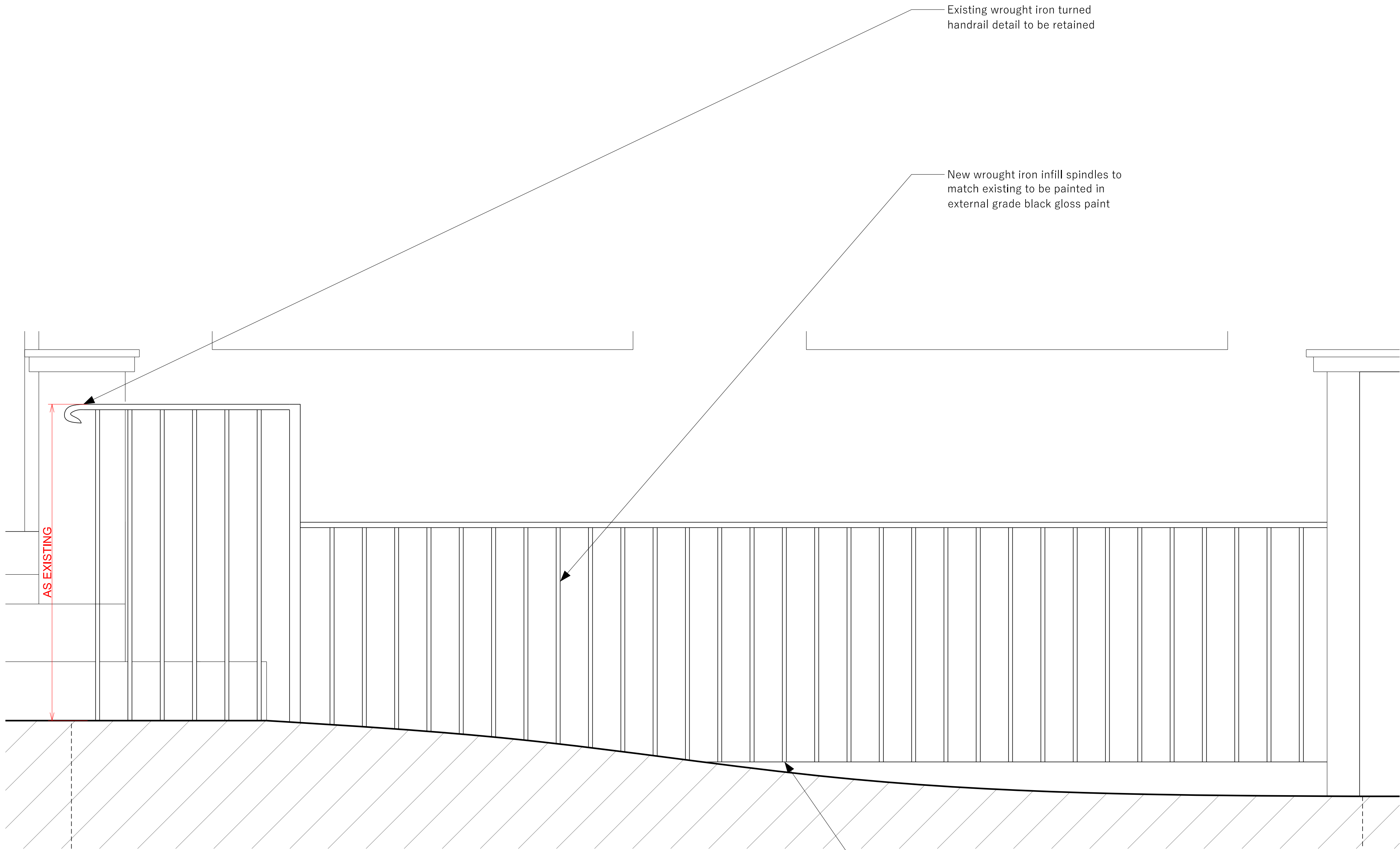
Proposed Front Railings Elevation
