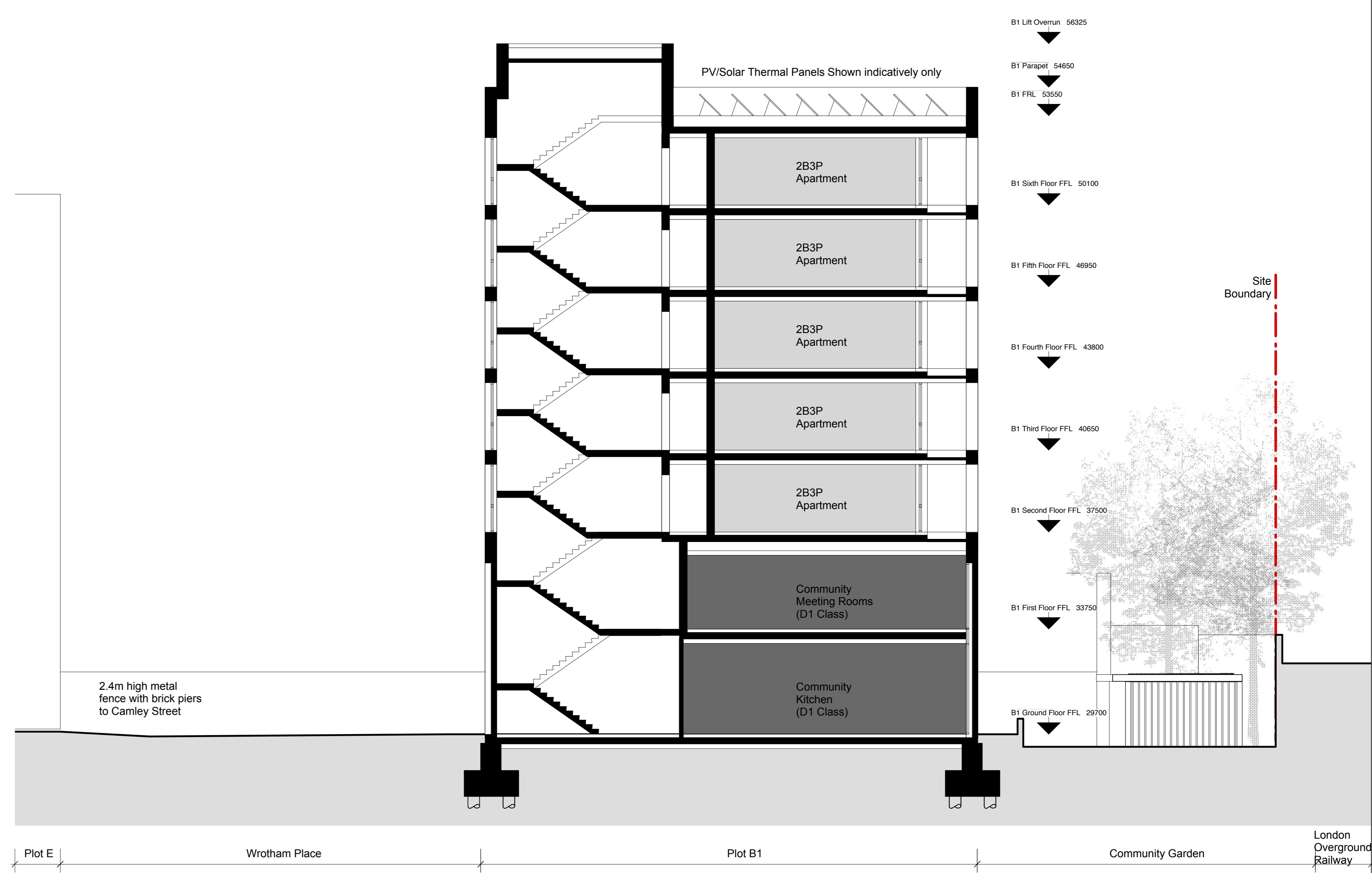
02 Section B Scale 1:100 @ A0
