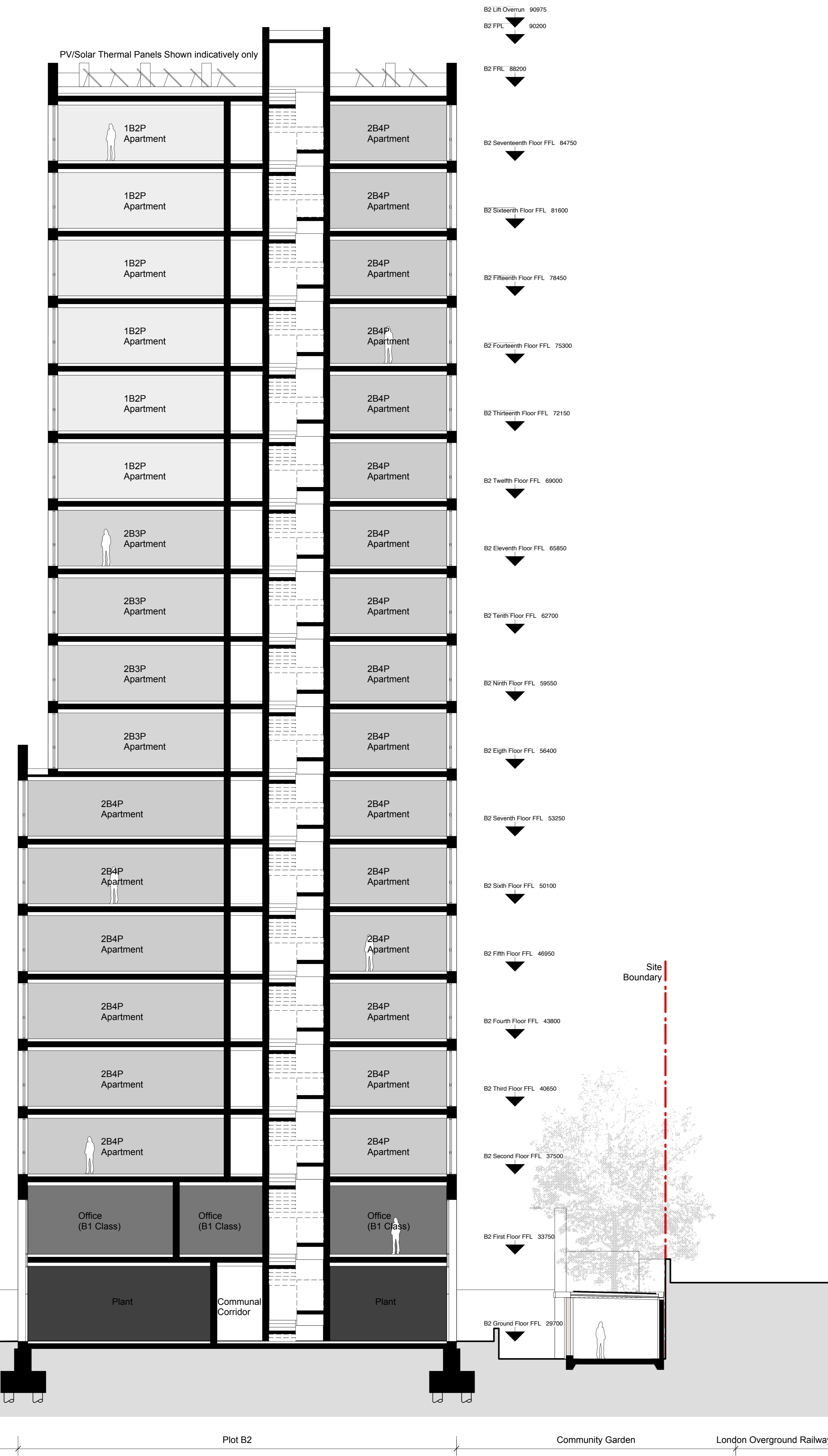
01 Section C Scale 1:100 @ A0
