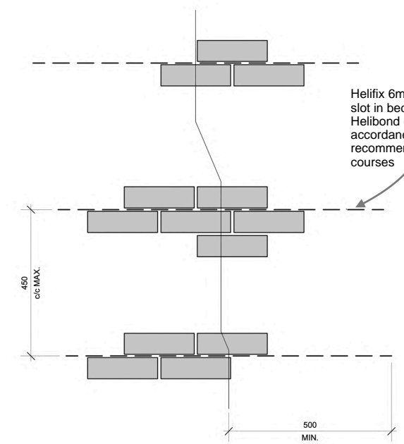
Crack Stitching at Location 'M'
