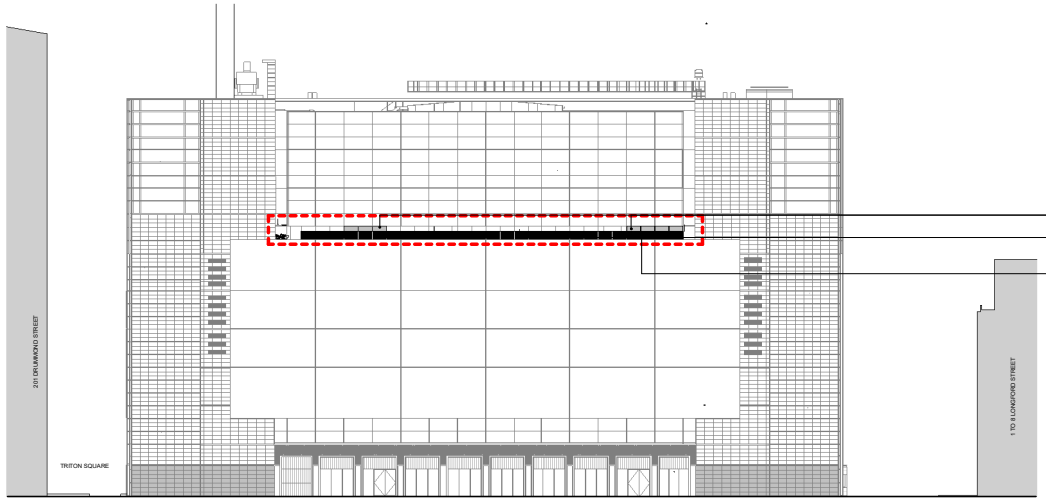
1 P004 - PROPOSED NORTH ELEVATION (LONGFORD STREET)
