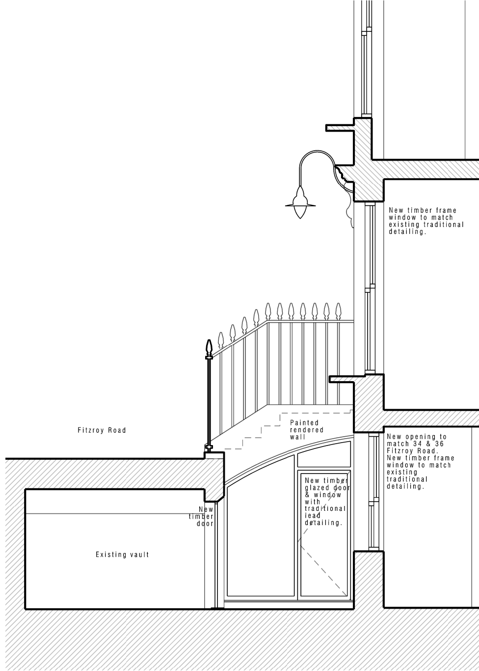
PROPOSED FRONT LIGHTWELL ELEVATION D
