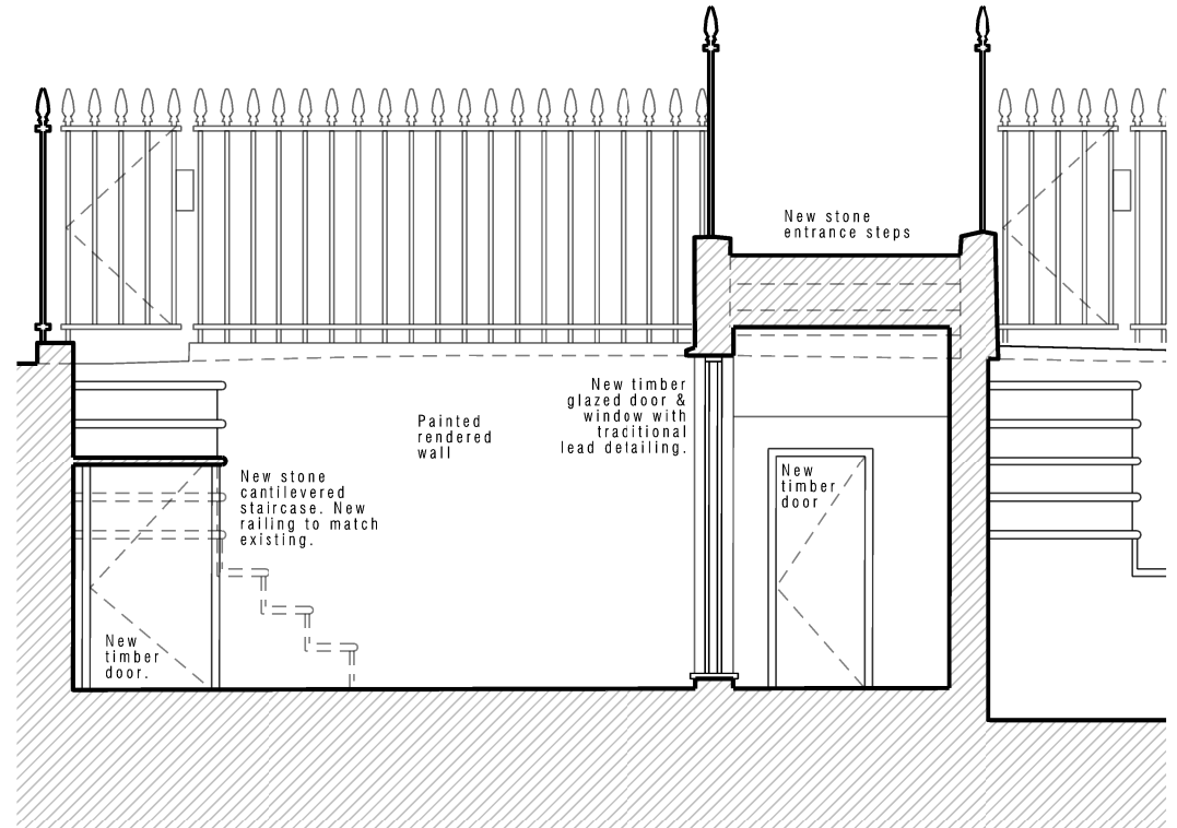
PROPOSED FRONT LIGHTWELL ELEVATION B
