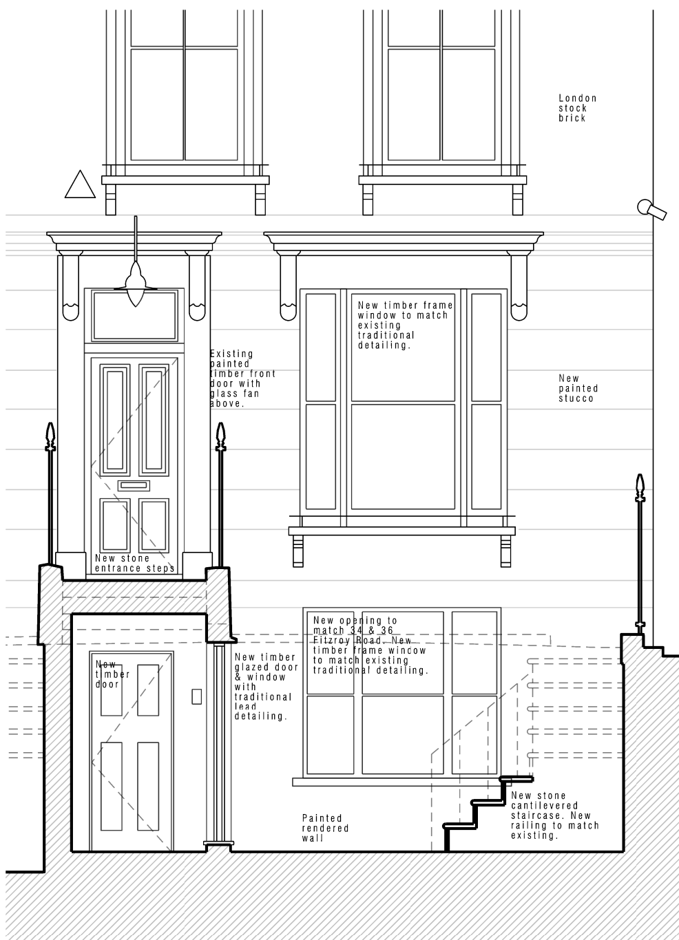
PROPOSED FRONT LIGHTWELL ELEVATION B
