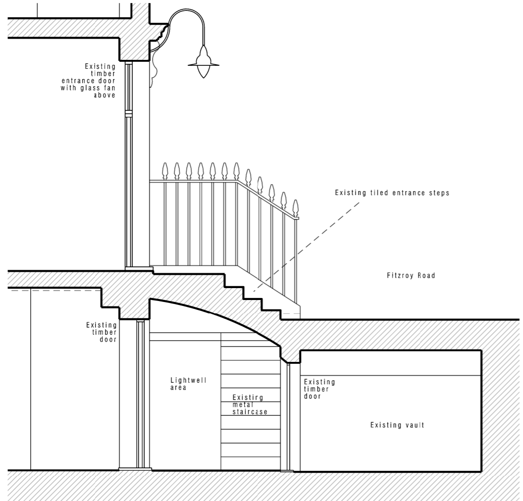
EXISTING ELEVATION A
