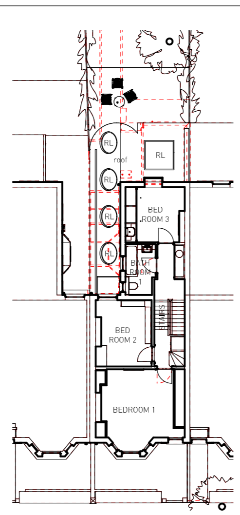
PROPOSED FIRST FLOOR PLAN 1:200
