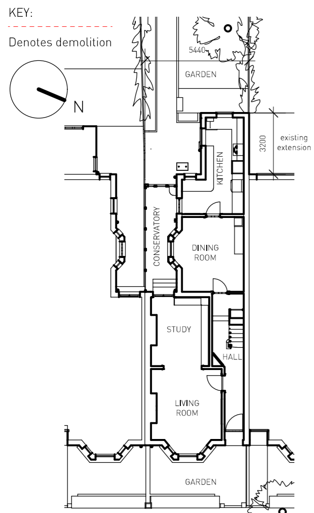
EXISTING GROUND FLOOR PLAN 1:200
