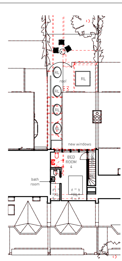
PROPOSED SECOND FLOOR PLAN 1:200
