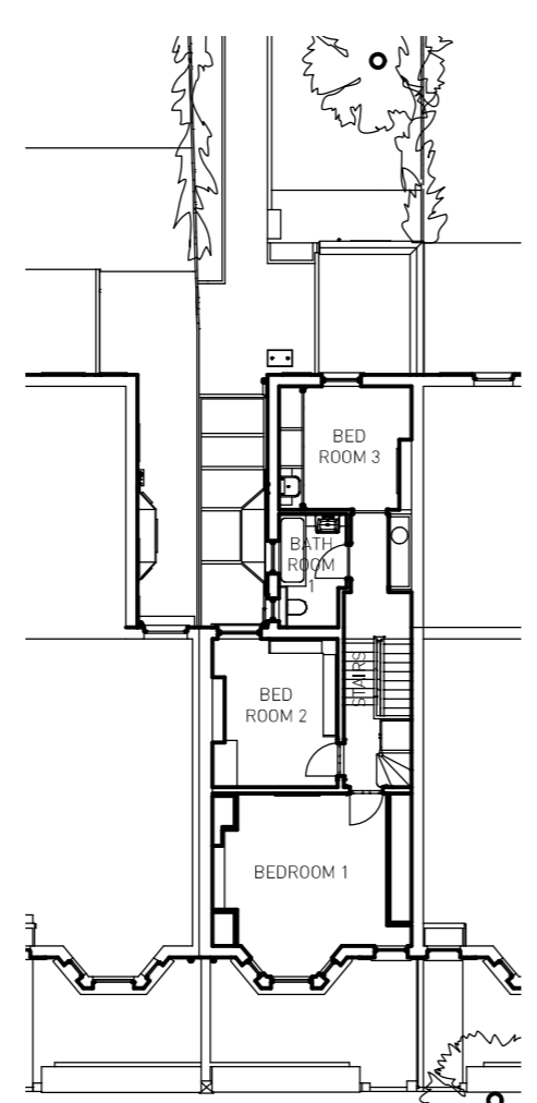
EXISTING FIRST FLOOR PLAN 1:200
