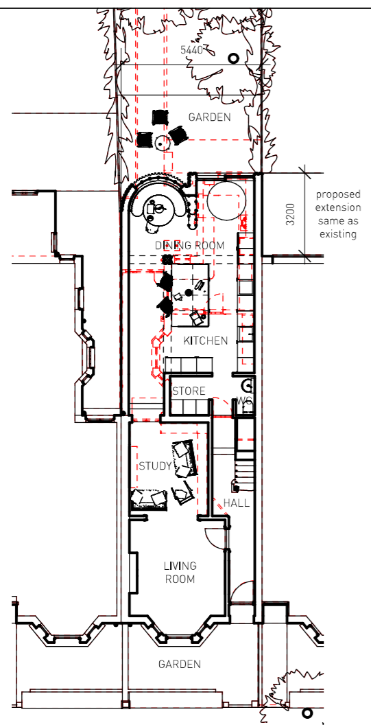
PROPOSED GROUND FLOOR PLAN 1:200
