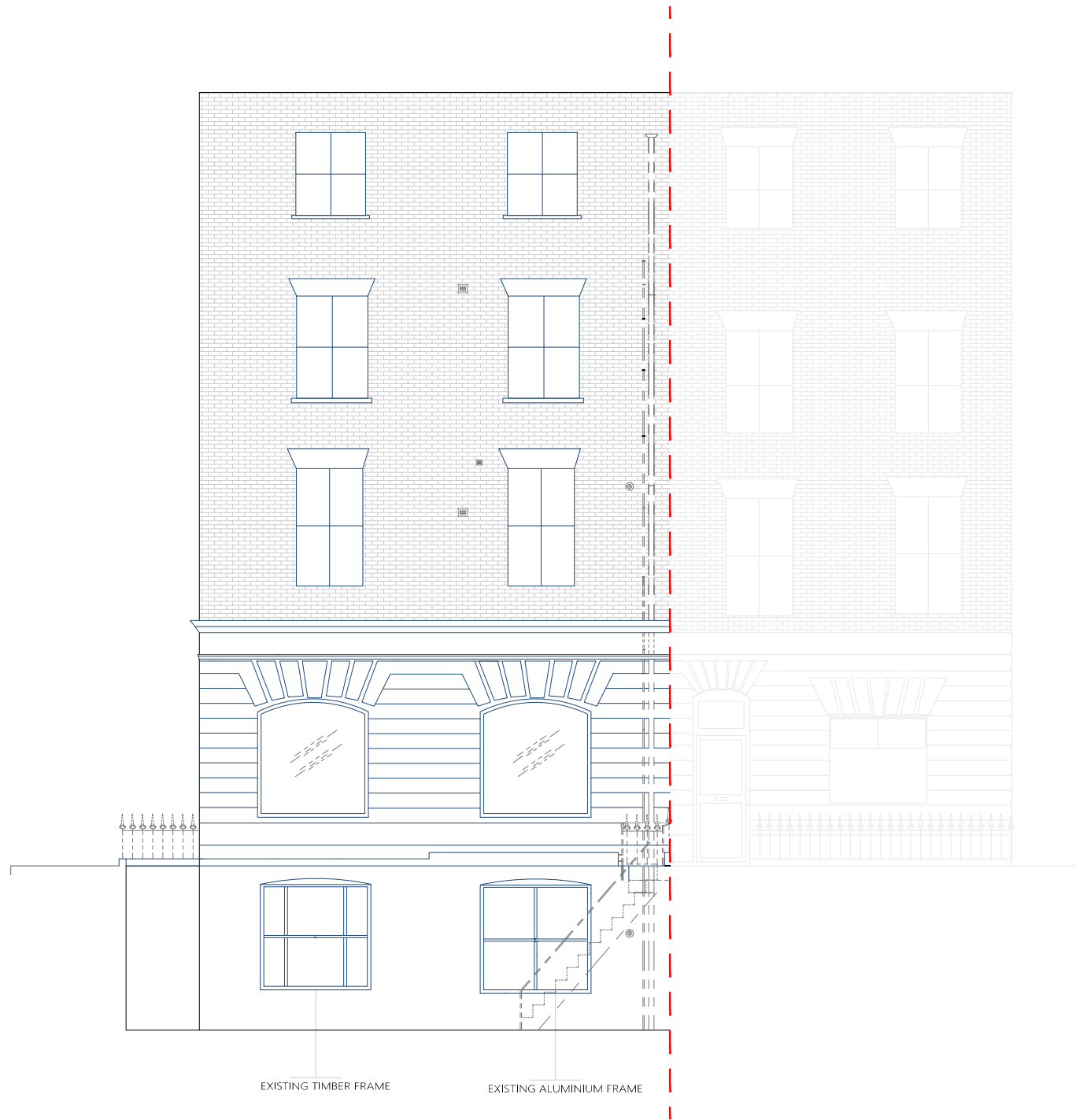
SIDE ELEVATION INC BASEMENT - TOTTENHAM STREET
