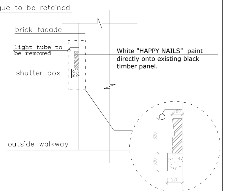
SECTION OF FRONT FACADE scale 1/100
