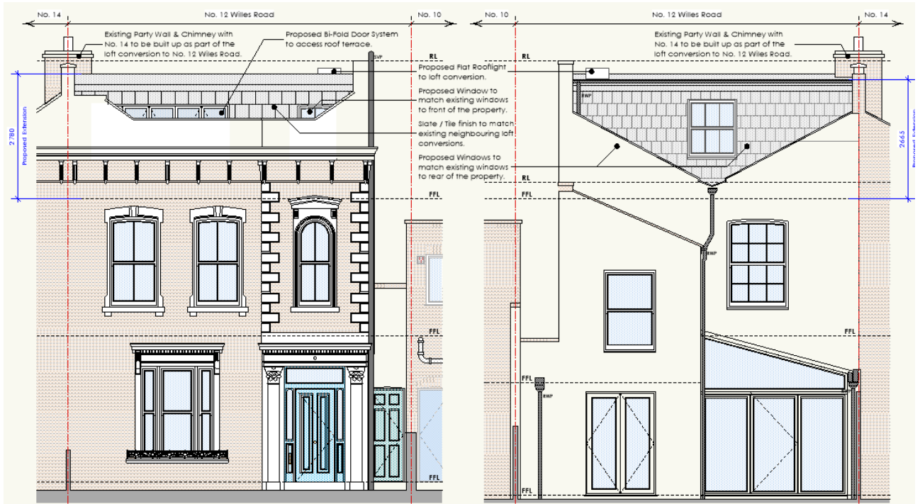
Fig. 3 Proposed Front Elevation
