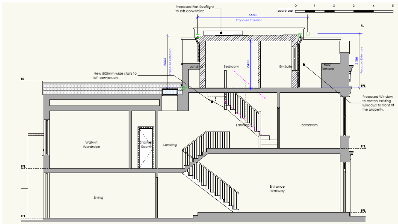
Fig. 5: Proposed Section [not to scale]
